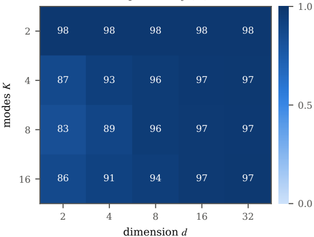
anchor round-trip accuracy (%), T=150
