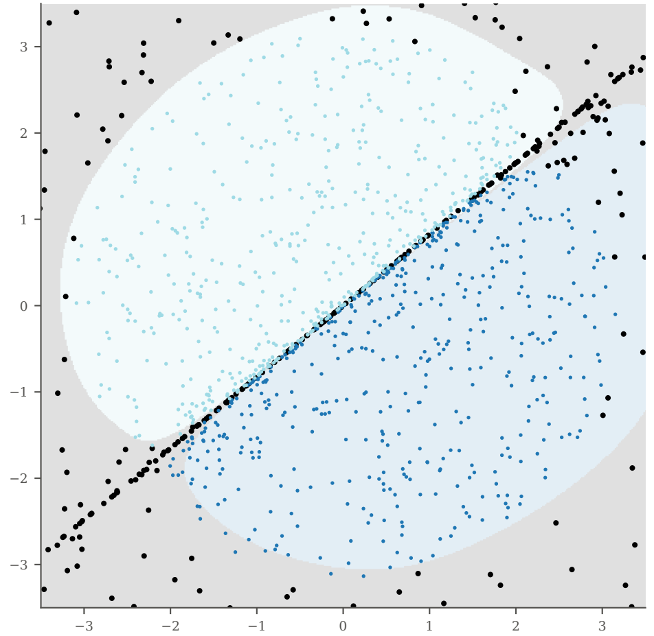
backtracked to SEED space (true score, T=200) over the learned fate map
