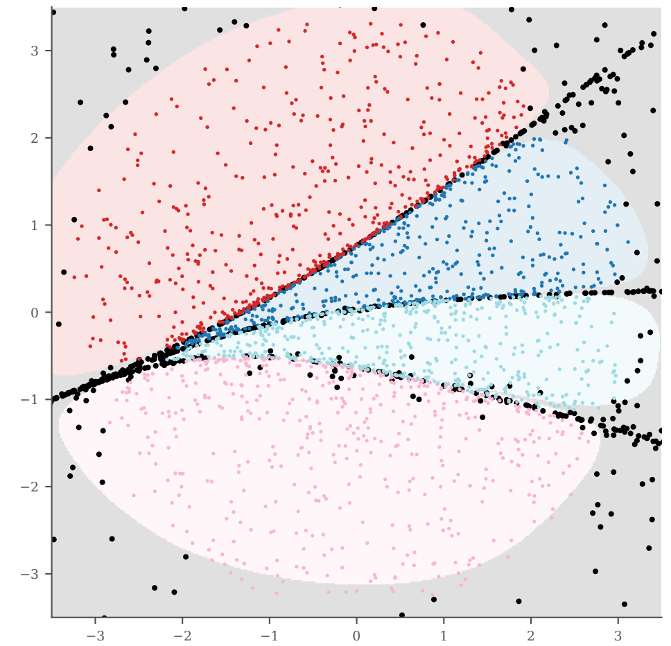
backtracked to SEED space (true score, T=300) over the learned fate map
