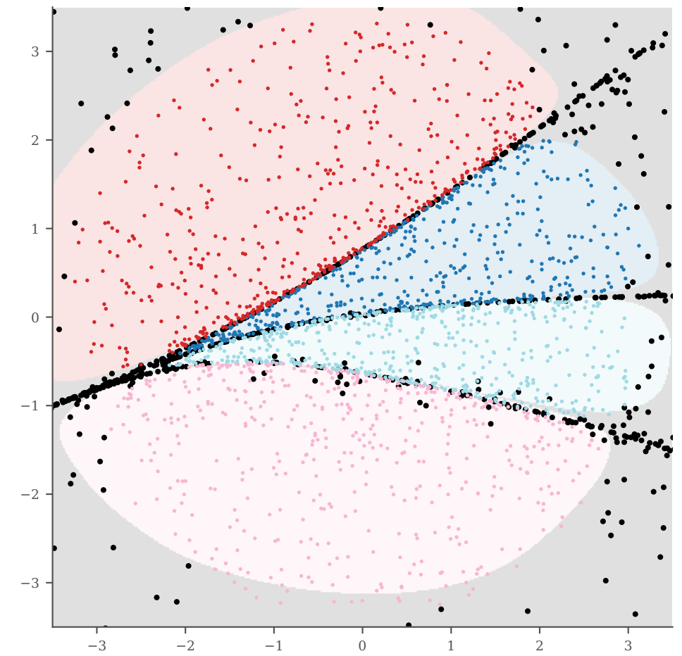
backtracked to SEED space (true score, T=350) over the learned fate map
