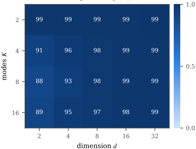
anchor round-trip accuracy (%), T=350
