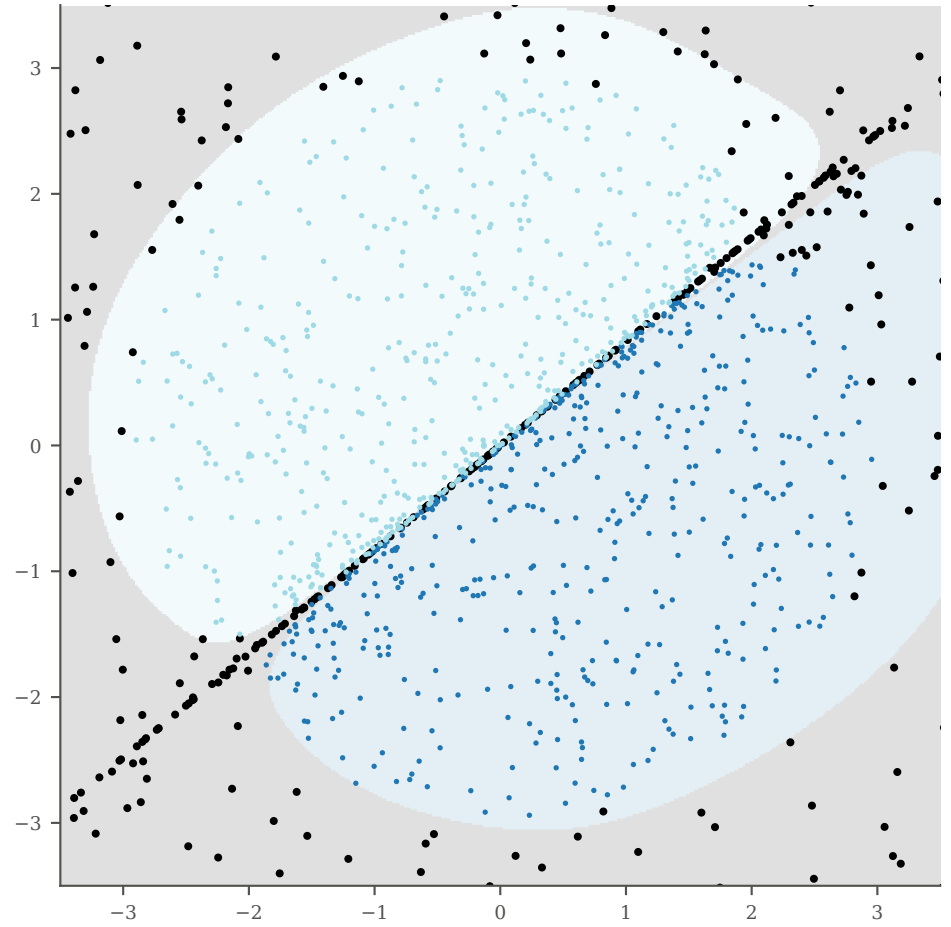
backtracked to SEED space (true score, T=50) over the learned fate map
