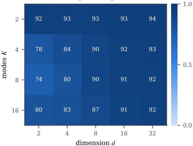
anchor round-trip accuracy (%), T=50
