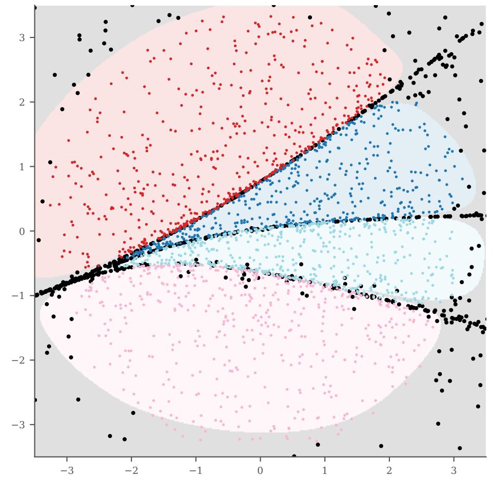
backtracked to SEED space (true score, T=500) over the learned fate map
