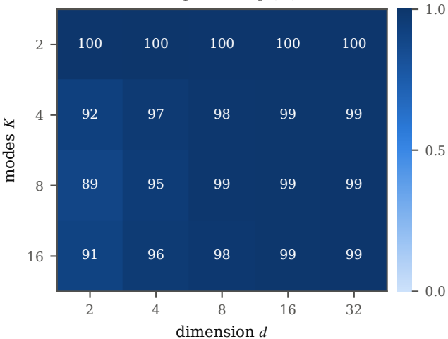
anchor round-trip accuracy (%), T=550
