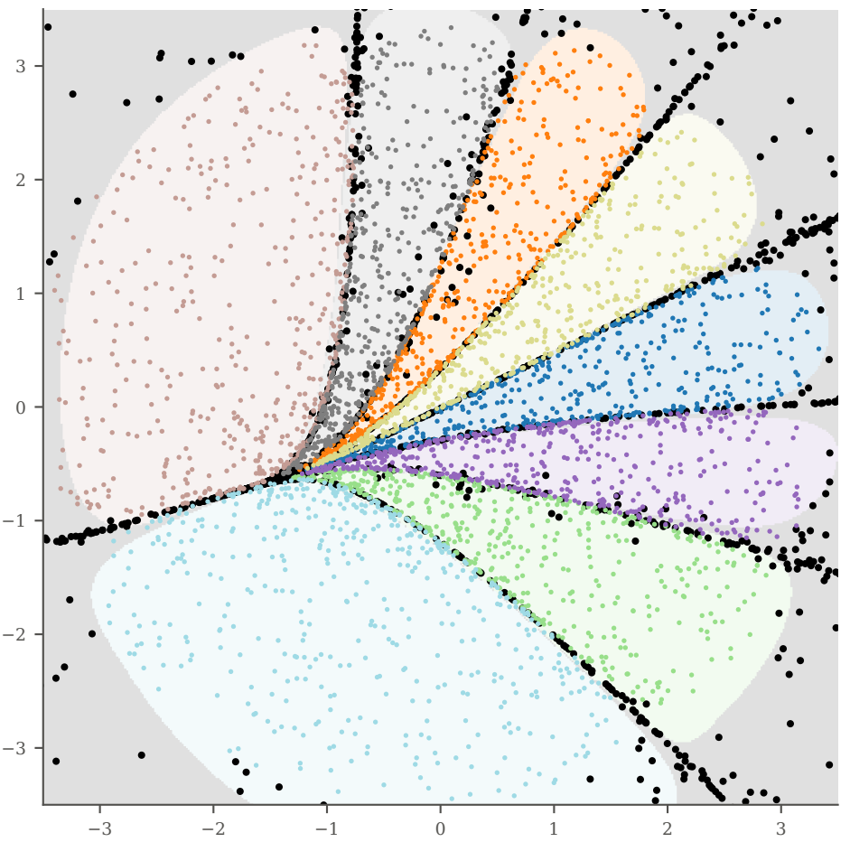
backtracked to SEED space (true score, T=650) over the learned fate map
