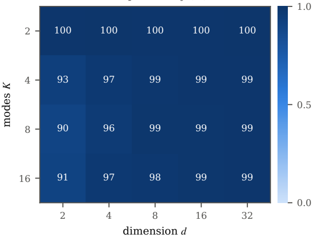
anchor round-trip accuracy (%), T=650
