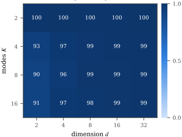
anchor round-trip accuracy (%), T=700
