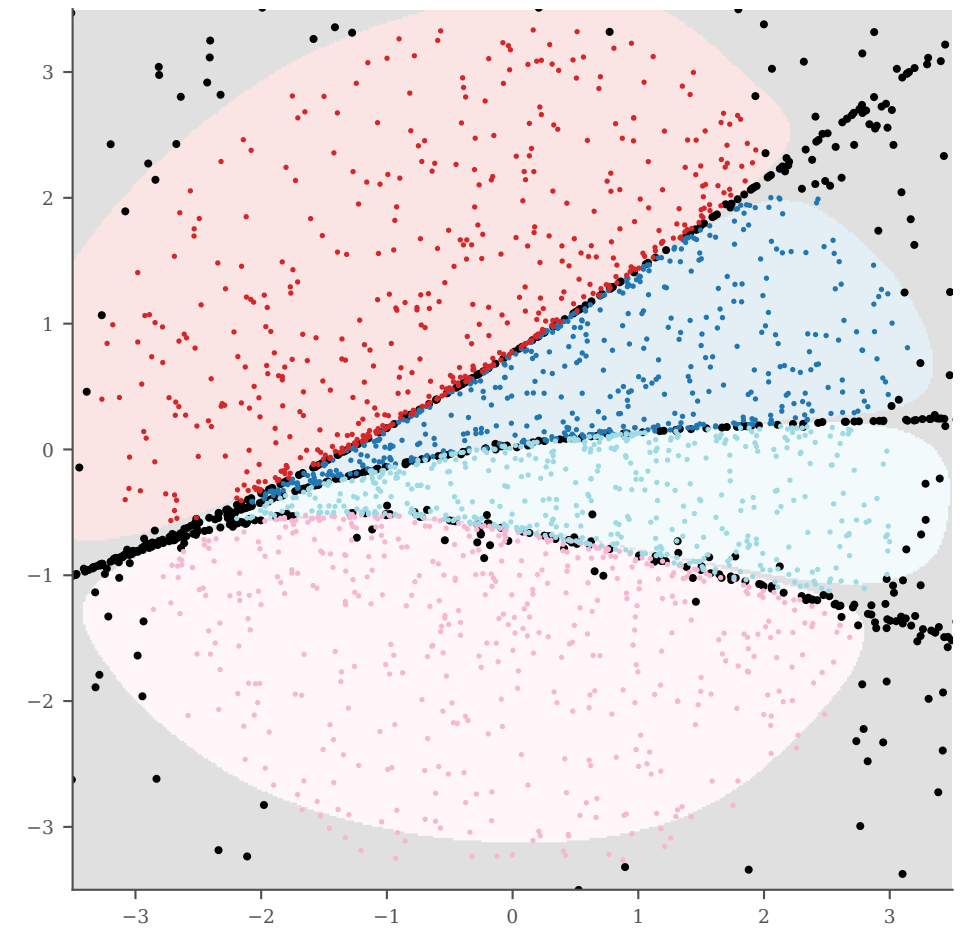
backtracked to SEED space (true score, T=750) over the learned fate map
