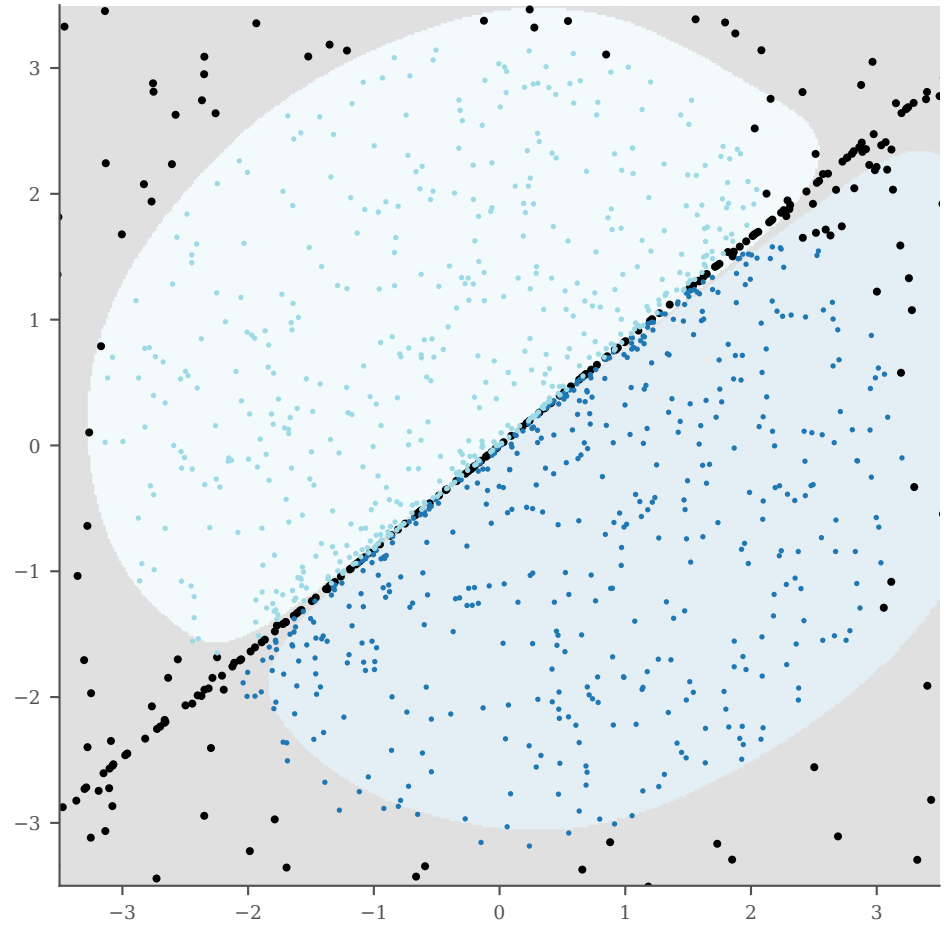
backtracked to SEED space (true score, T=800) over the learned fate map
