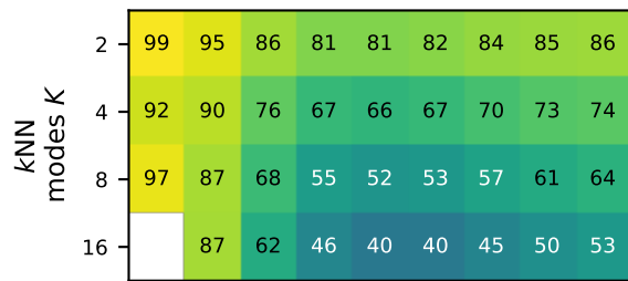
overall accuracy
