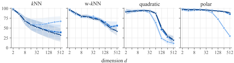
RK45 accuracy (%)
