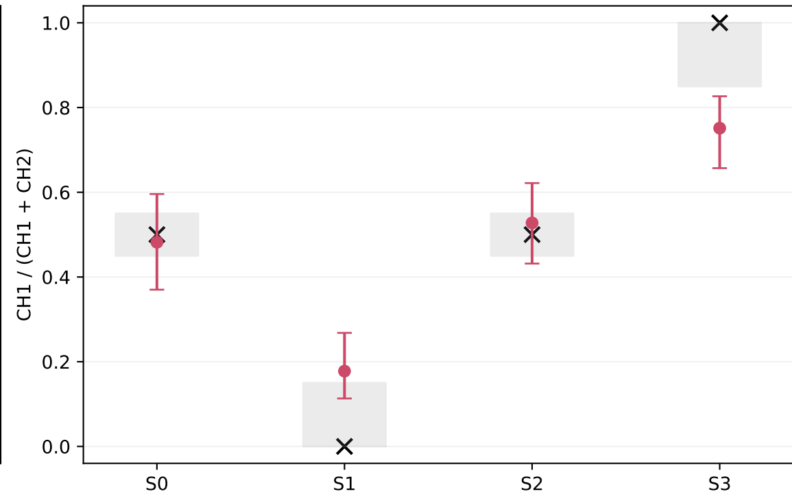
Bob setting 2: -54.545 V
