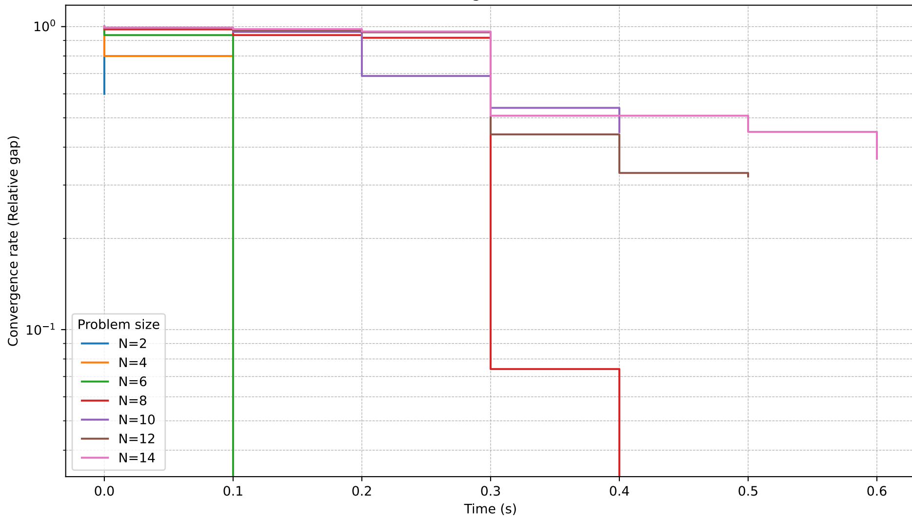
MOSEK convergence rate vs. time
