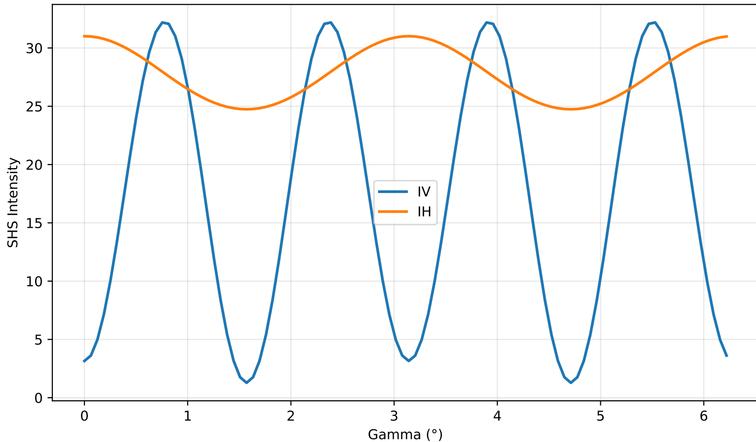
Polarization-resolved SHS
