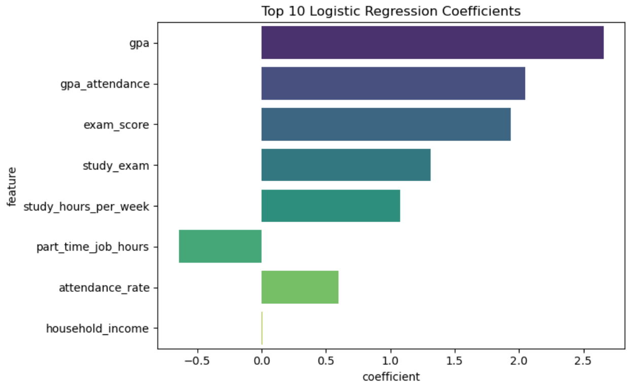
Figure 11. Top Logistic Regression coefficients. Academic features dominate.
