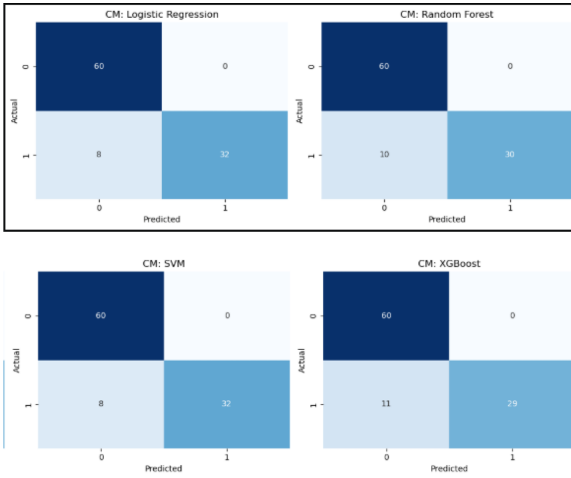
Figure 7. Confusion matrices show identical precision but varying recall across models.
