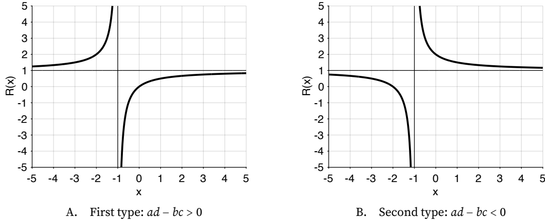
FIGURE F.1. The two types of linear-over-linear rational functions
