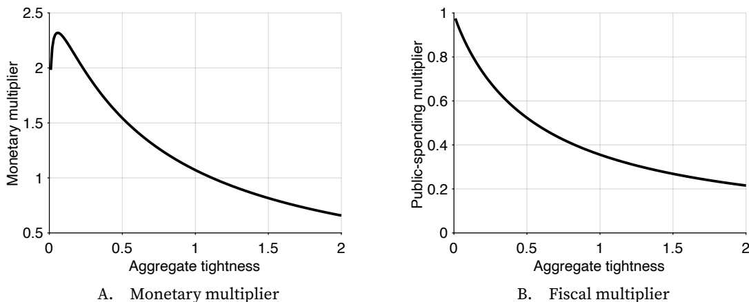
FIGURE 13.5. Policy multipliers in the slackish business cycle model
