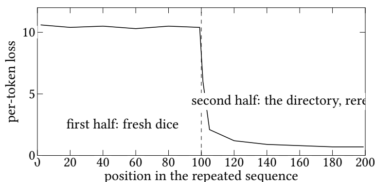
Exhibit 3.2 (The telephone-directory signature). Per-token loss over a repeated random sequence: dismal by construction in the first half, collapsing at the splice – and the collapse is attributable, by the census and the ablation, to the certified heads. Schematic placeholder: the assembled volume prints Lab 3.1’s measured curve on GPT-2 small, with the certified heads named by coordinate.
