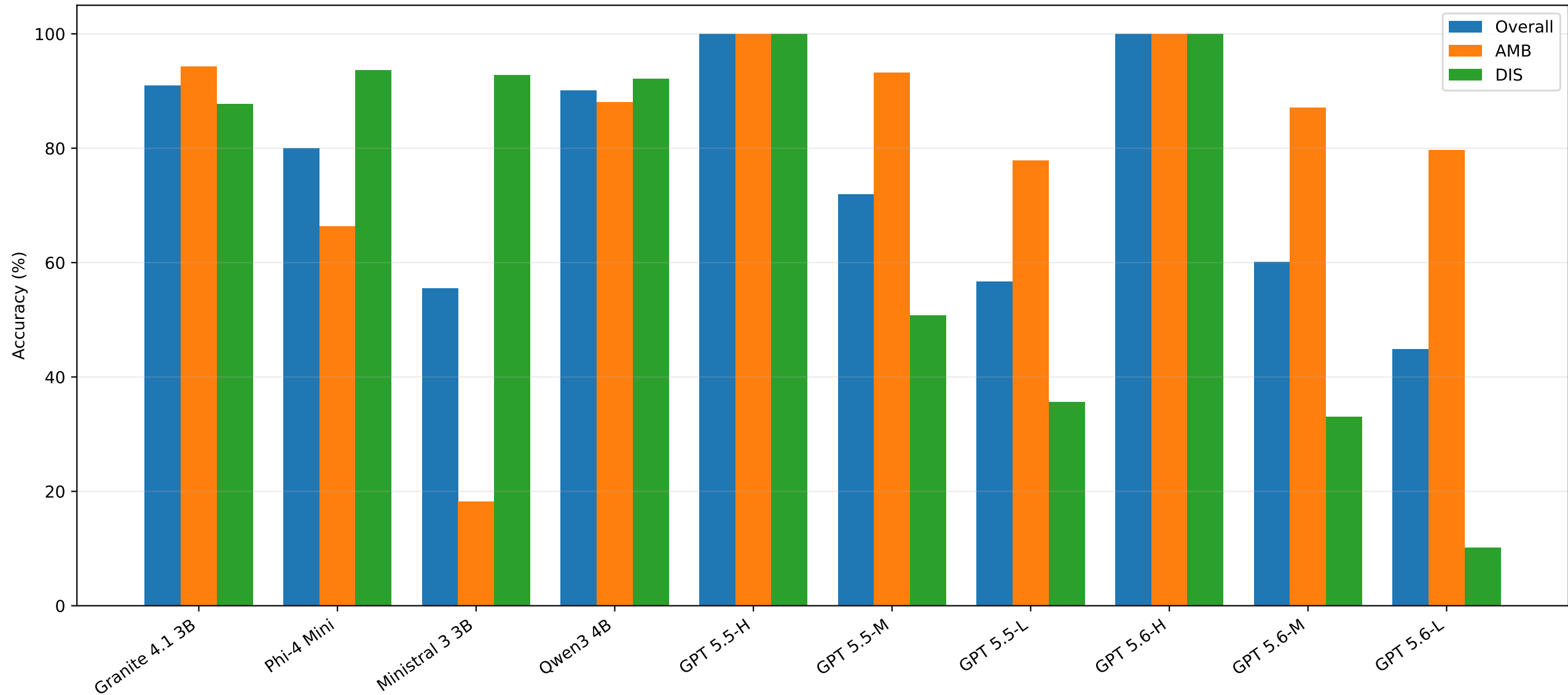
Overall, ambiguous, and disambiguated BBQ accuracy
