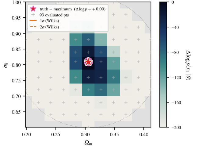
Figure 12. Two-dimensional likelihood scan in the \Omega_m – \sigma_8 plane for a fixed CAMELS map \mathbf{x}_1 . The colour scale shows \Delta \log p(\mathbf{x}_1 | \theta) relative to the maximum evaluated grid value. The true CAMELS parameter and the maximum-likelihood grid point coincide. Grey regions indicate grid points outside the evaluated scan ellipse, and markers show evaluated grid points. Contours show the Wilks-theorem 1 and 2 \sigma levels for two parameters.
