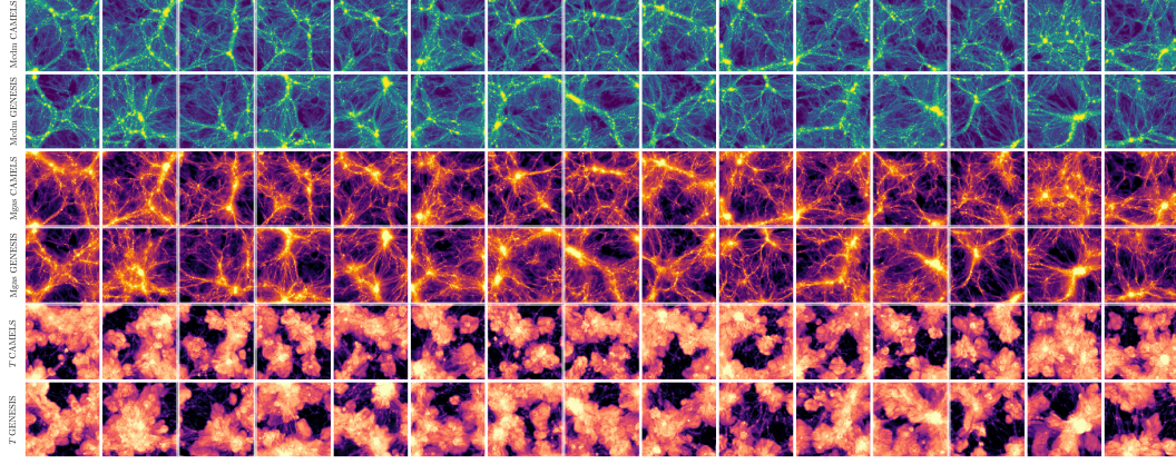
Figure C7. LH 0142: (\Omega_m, \sigma_8, A_{\text{SN1}}, A_{\text{SN2}}, A_{\text{AGN1}}, A_{\text{AGN2}}) = (0.425, 0.810, 0.274, 1.696, 0.621, 1.477) . Each tile arranges 15 generated samples with the corresponding CAMELS reference rows.
