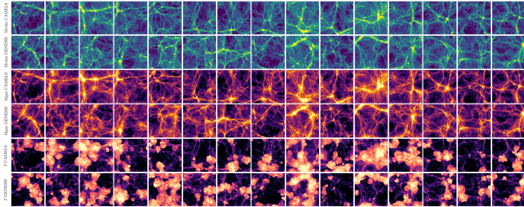
Figure C3. LH 0015: (\Omega_m, \sigma_8, A_{\text{SN1}}, A_{\text{SN2}}, A_{\text{AGN1}}, A_{\text{AGN2}}) = (0.218, 0.788, 0.825, 0.274, 0.552, 1.106) . Each tile arranges 15 generated samples with the corresponding CAMELS reference rows.
