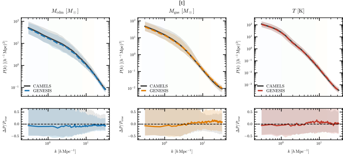
Figure 8. Auto-power spectra on the CV set. Top panels show CAMELS and GENESIS auto-power spectra for M_{\text{cdm}} , M_{\text{gas}} , and T ; shaded regions indicate the 16–84 percentile ranges. Bottom panels show fractional residuals relative to the CAMELS median.
