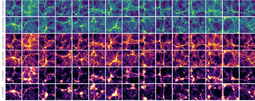
Figure C2. LH 0218: (\Omega_m, \sigma_8, A_{\text{SN1}}, A_{\text{SN2}}, A_{\text{AGN1}}, A_{\text{AGN2}}) = (0.150, 0.743, 0.924, 0.342, 1.030, 0.523) . Each tile arranges 15 generated samples with the corresponding CAMELS reference rows.
