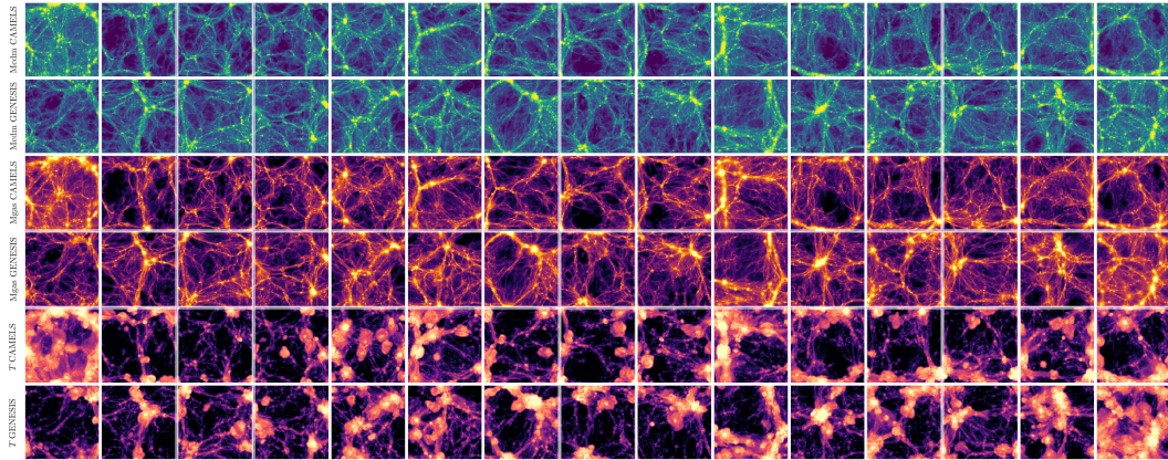
Figure C9. LH 0108: (\Omega_m, \sigma_8, A_{\text{SN1}}, A_{\text{SN2}}, A_{\text{AGN1}}, A_{\text{AGN2}}) = (0.499, 0.630, 1.310, 2.385, 0.518, 0.623) . Each tile arranges 15 generated samples with the corresponding CAMELS reference rows.
