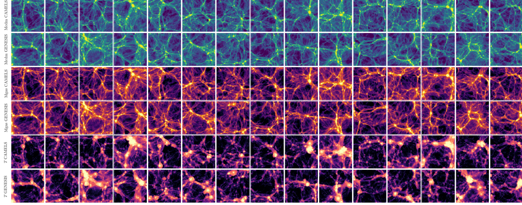
Figure C4. LH 0074: (\Omega_m, \sigma_8, A_{SN1}, A_{SN2}, A_{AGN1}, A_{AGN2}) = (0.282, 0.724, 1.587, 0.270, 1.330, 0.990) . Each tile arranges 15 generated samples with the corresponding CAMELS reference rows.
