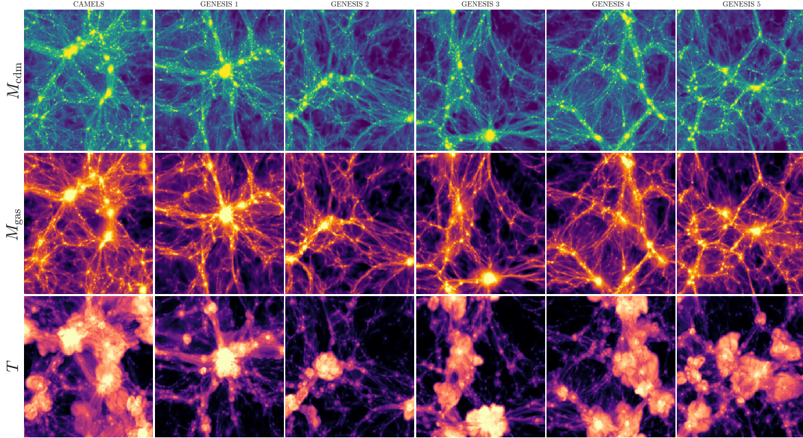
Figure 7. Comparison between CAMELS CV maps and GENESIS-generated maps, conditioned on (\Omega_m, \sigma_8, A_{SN1}, A_{SN2}, A_{AGN1}, A_{AGN2}) = (0.30, 0.80, 1, 1, 1, 1) . CAMELS realizations are compared with independent GENESIS samples generated at the same conditioning vector. Rows show M_{\text{cdm}} , M_{\text{gas}} , and T .
