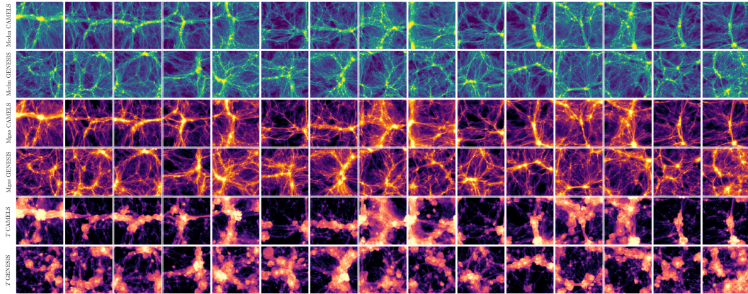
Figure C6. LH 0008: (\Omega_m, \sigma_8, A_{SN1}, A_{SN2}, A_{AGN1}, A_{AGN2}) = (0.389, 0.778, 0.287, 0.258, 1.699, 1.036) . Each tile arranges 15 generated samples with the corresponding CAMELS reference rows.
