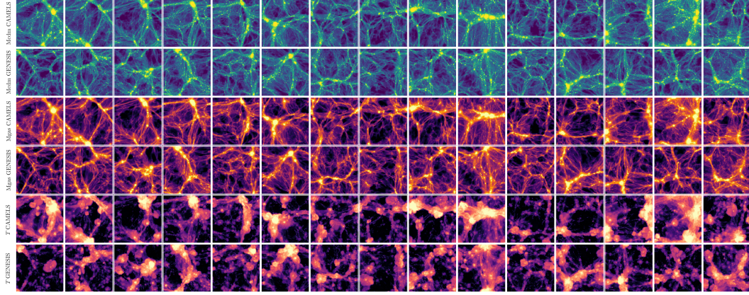
Figure C8. LH 0479: (\Omega_m, \sigma_8, A_{\text{SN1}}, A_{\text{SN2}}, A_{\text{AGN1}}, A_{\text{AGN2}}) = (0.462, 0.940, 0.993, 0.433, 1.762, 1.469) . Each tile arranges 15 generated samples with the corresponding CAMELS reference rows.
