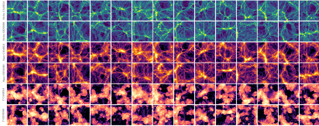
Figure C5. LH 0163: (\Omega_m, \sigma_8, A_{SN1}, A_{SN2}, A_{AGN1}, A_{AGN2}) = (0.337, 0.950, 0.577, 1.705, 0.670, 1.077) . Each tile arranges 15 generated samples with the corresponding CAMELS reference rows.
