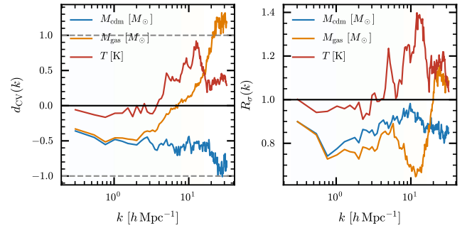
Figure 9. CV-normalized spectral displacement and map-level spread. Left: d_{\text{CV}}(k) for the generated mean auto-power spectrum. Right: R_{\sigma}(k) , the ratio of generated to CAMELS map-level log-power variance.
