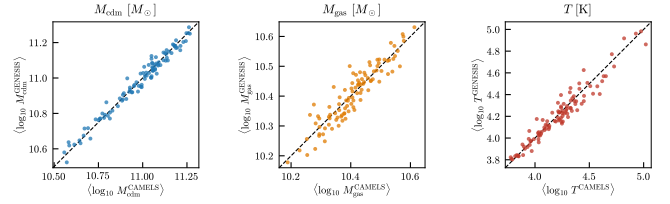
Figure 4. Per-simulation mean field values on the LH test set. Each point corresponds to one held-out conditioning vector. The dashed line marks the one-to-one relation between CAMELS and GENESIS.
