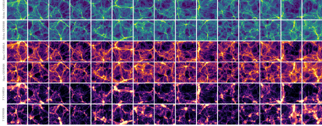
Figure C1. LH 0719: (\Omega_m, \sigma_8, A_{\text{SN1}}, A_{\text{SN2}}, A_{\text{AGN1}}, A_{\text{AGN2}}) = (0.104, 0.747, 3.308, 0.446, 1.461, 0.549) . Each tile arranges 15 generated samples with the corresponding CAMELS reference rows.
