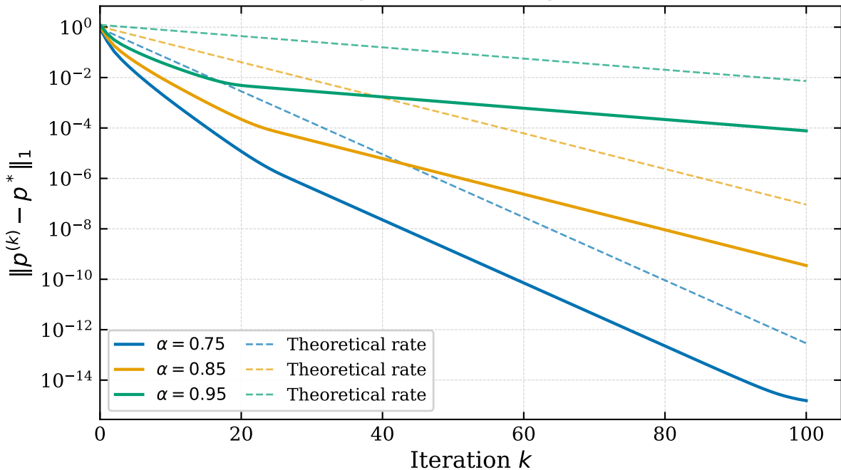
PageRank convergence
