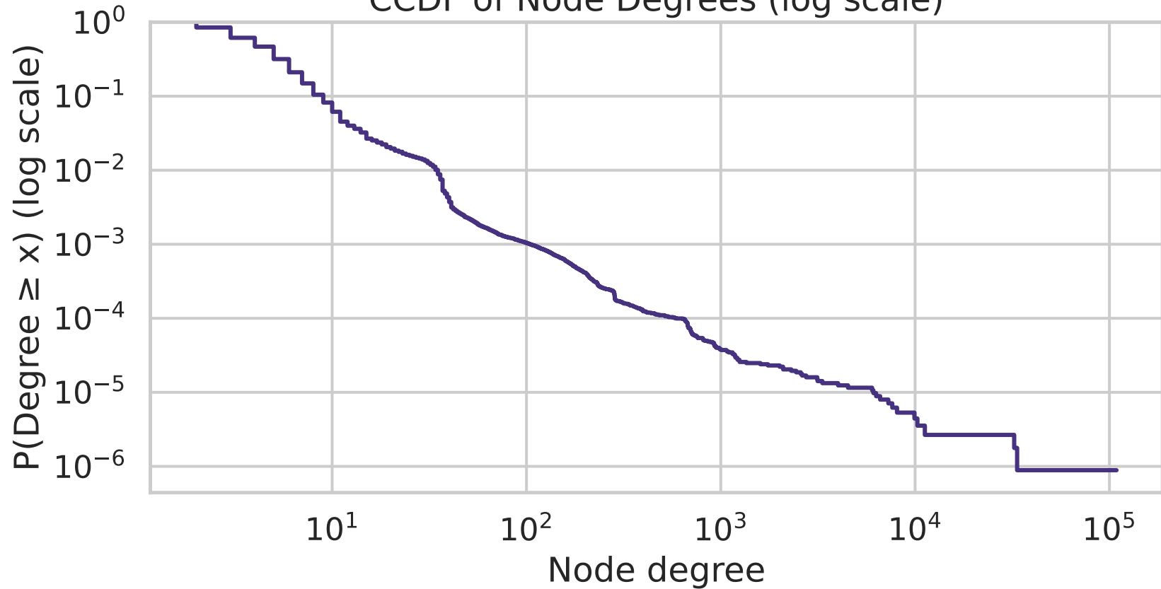
CCDF of Node Degrees (log scale)
