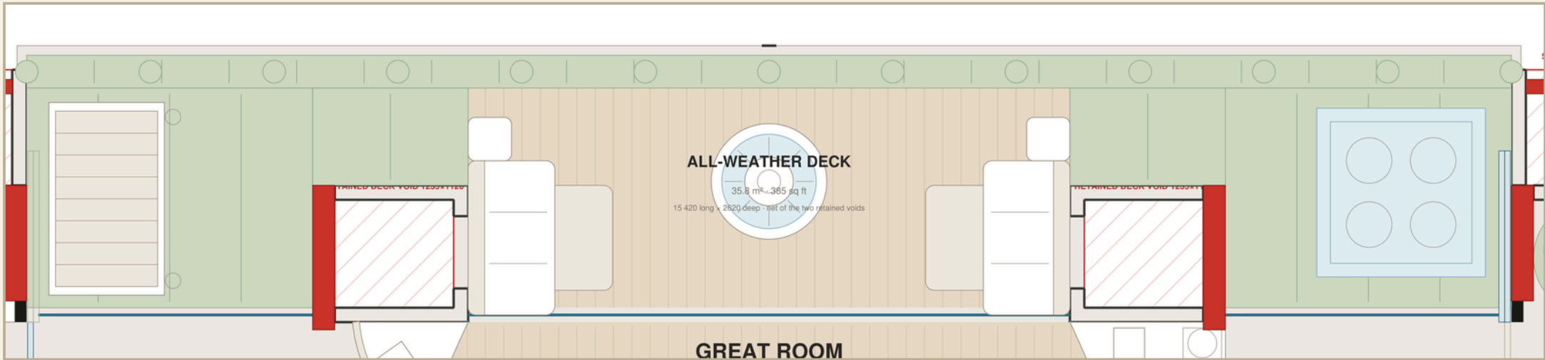
from the working plan — true to scale
