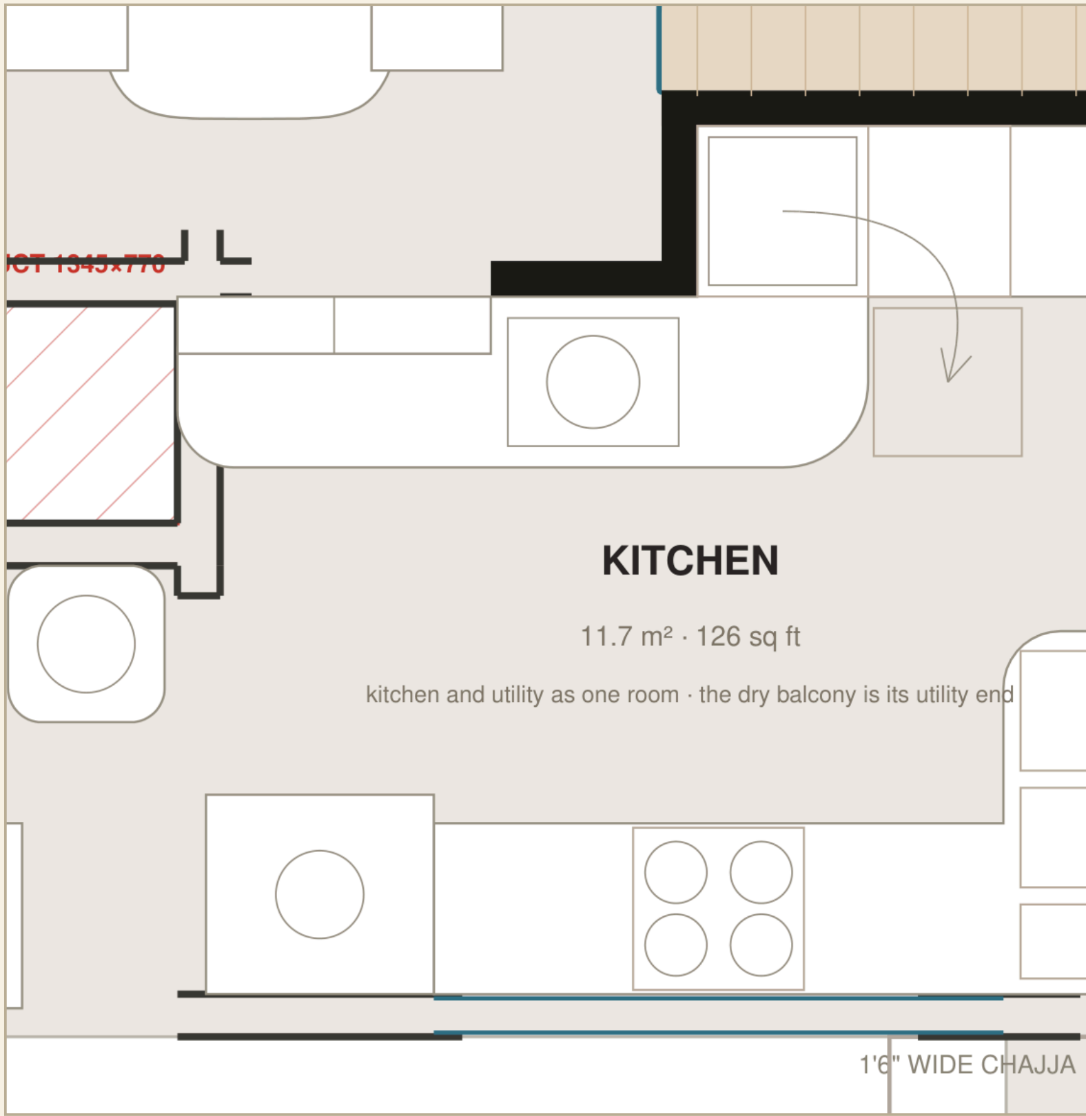
from the working plan — true to scale
