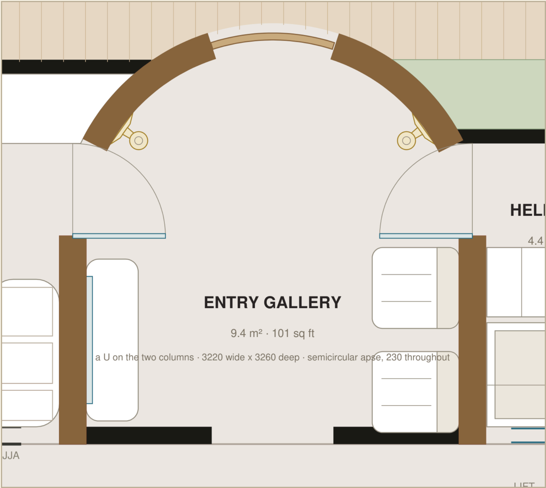
from the working plan — true to scale
