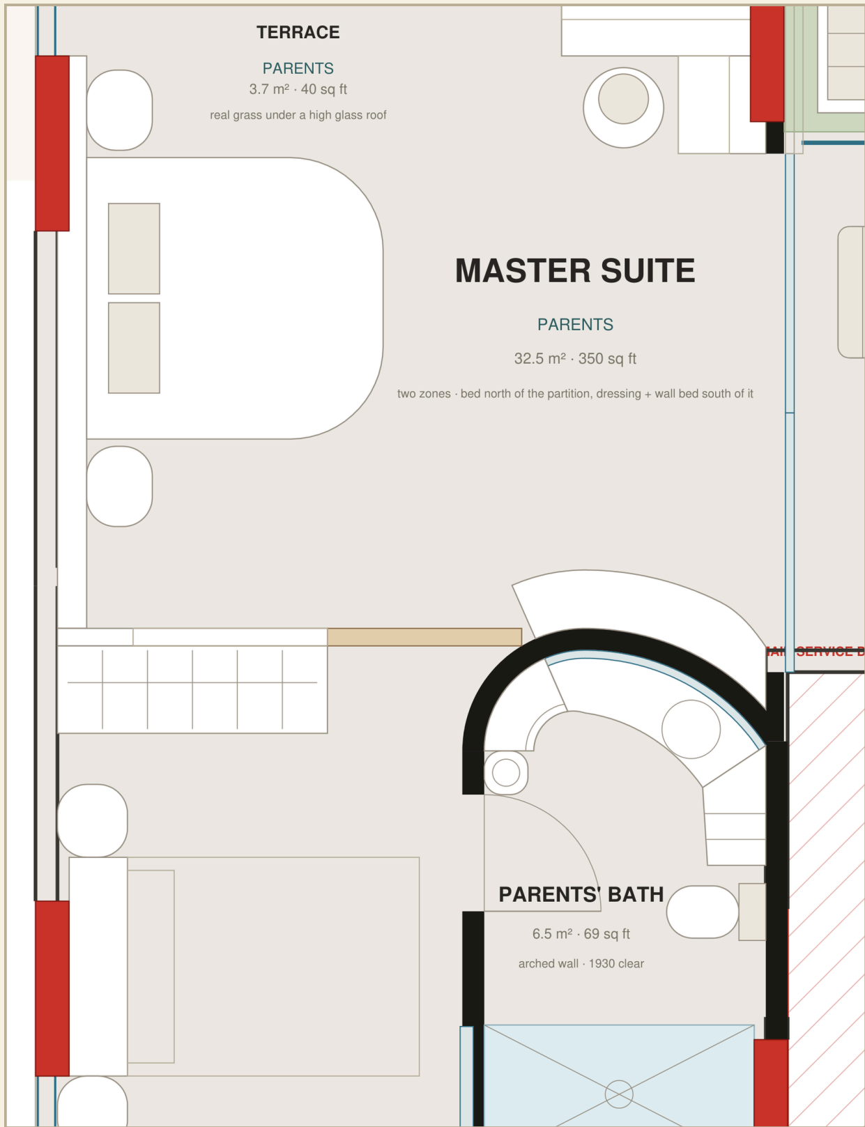
from the working plan — true to scale
