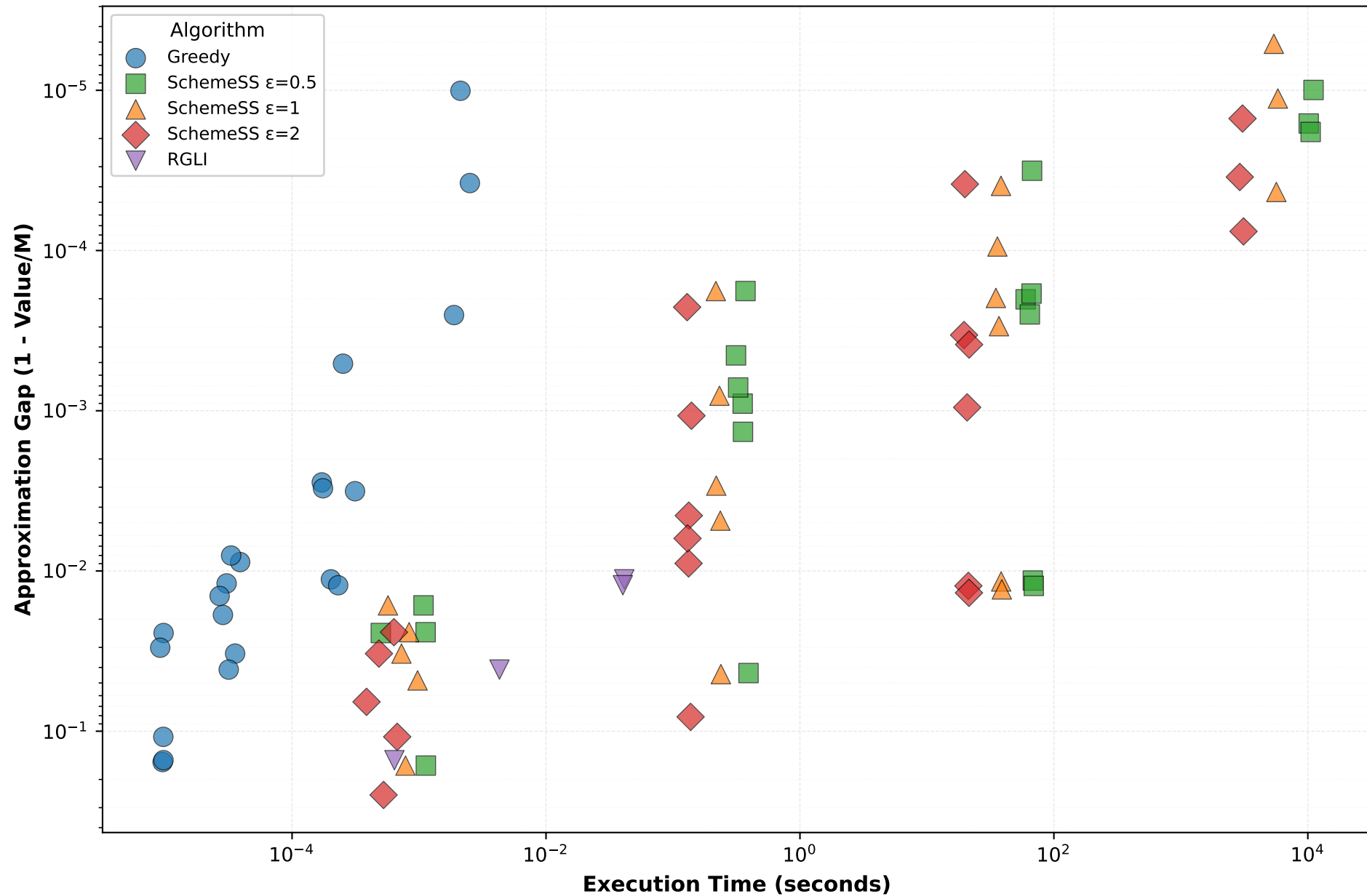
Algorithm Performance: Time vs Quality Trade-off
