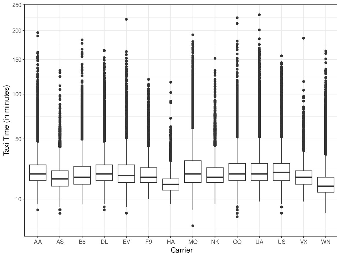
Figure 15.4: A box plot
