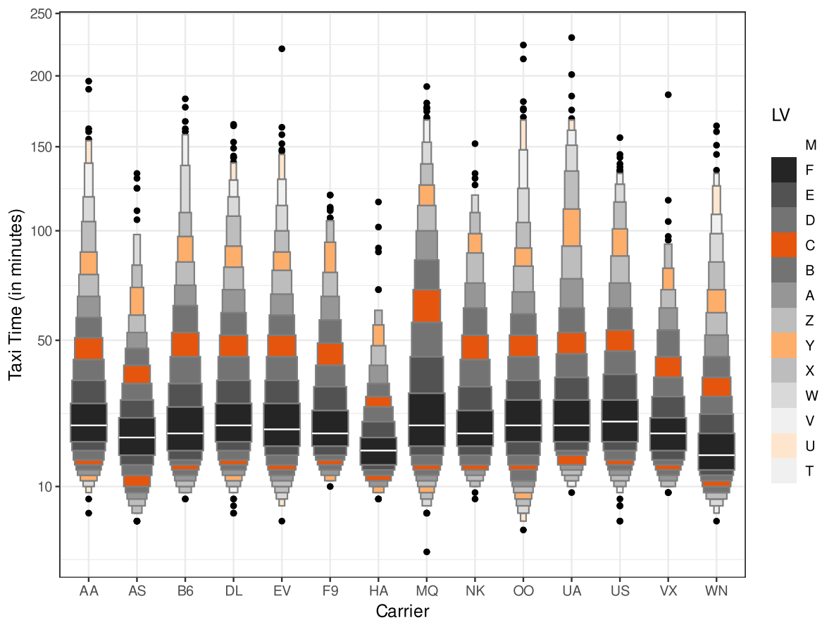
Figure 15.3: A letter-value plot
