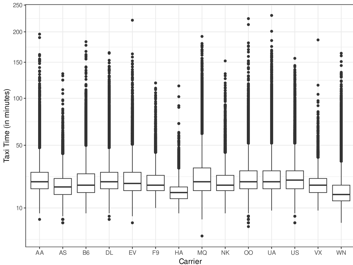
Figure 14.15: A box plot
