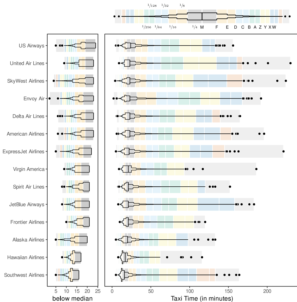
Figure 14.16: An improved letter-value plot?
