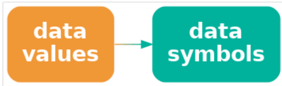
Figure 1.3: A data visualisation is largely defined by the mappings that it uses to represent data values as data symbols .
