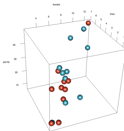
Figure 11.8: A data visualisation of three RWC variables
