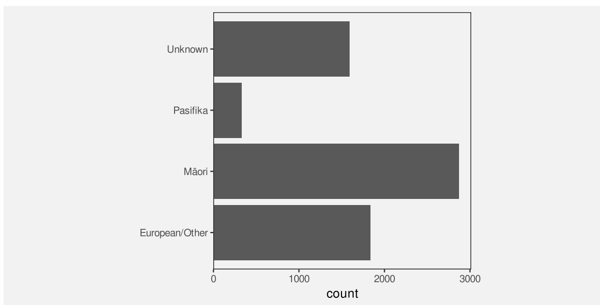
Figure 3.2: A bar plot of the total number of offenders for different ethnic groups in 2021. The data symbols in this plot are the horizontal bars.
