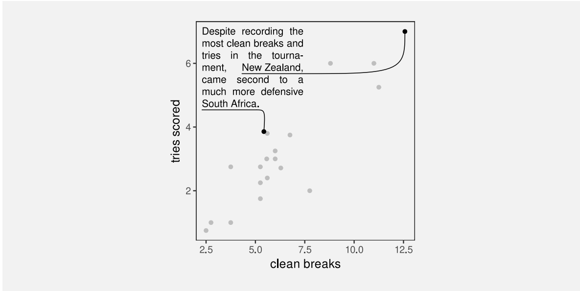
Figure 13.7: The number of times a team breaks through the opposition defence and the number of tries that a team scores (both are per-game averages) for teams in the 2023 Rugby World Cup.
