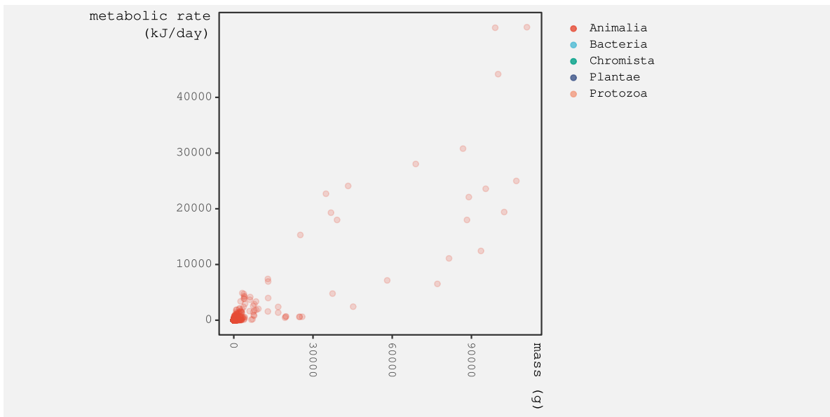
Figure 10.20: Body mass versus metabolic rate for a wide variety of lifeforms.
