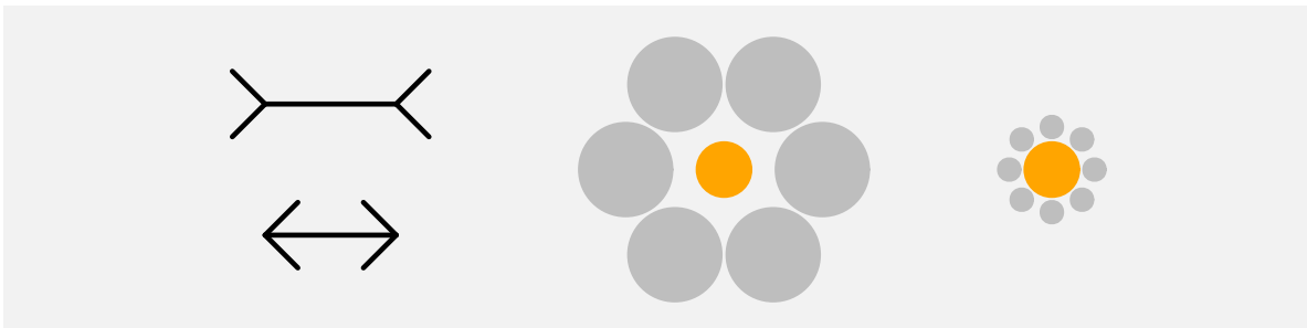
Figure 2.22: The two horizontal lines in the Muller-Lyer illusion on the left have exactly the same physical length, but the top line appears longer. The two orange circles in the Ebbinghaus illusion on the right have exactly the same physical radius, but they appear to be different sizes.
