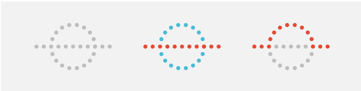
Figure 2.16: What shapes emerge from the collection of points on the left? We have a preference for completing curves and straight lines (in the middle) rather than shapes with sharp corners (on the right).
