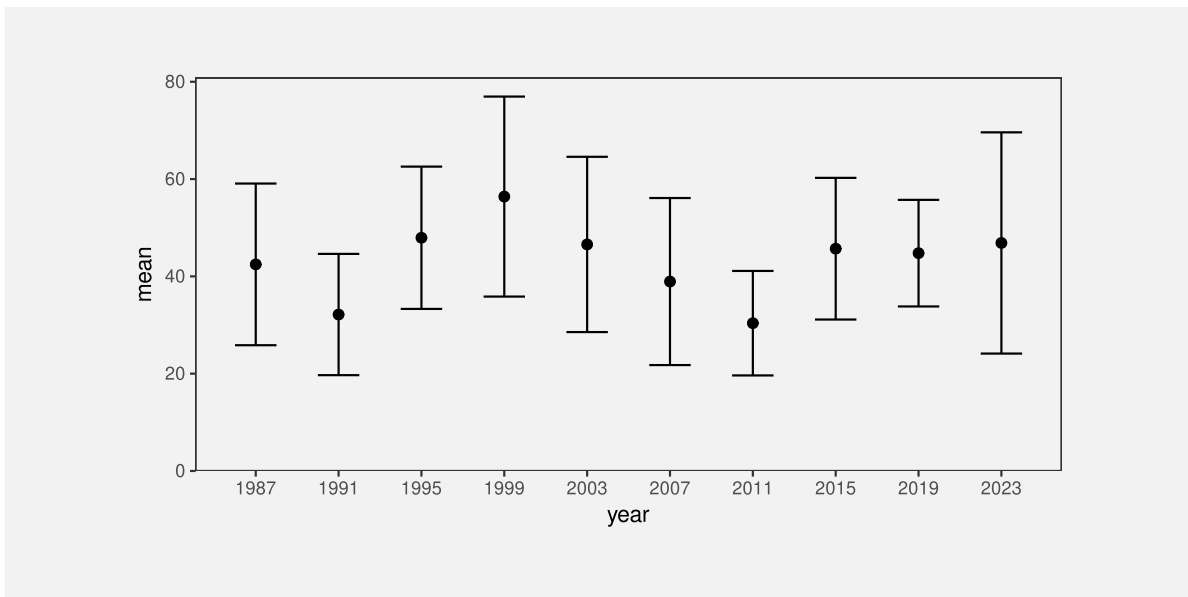
Figure 8.20: A plot of the mean points scored, plus-or-minus the standard deviations of points scored, in matches between Tier One nations at Rugby World Cup matches.
