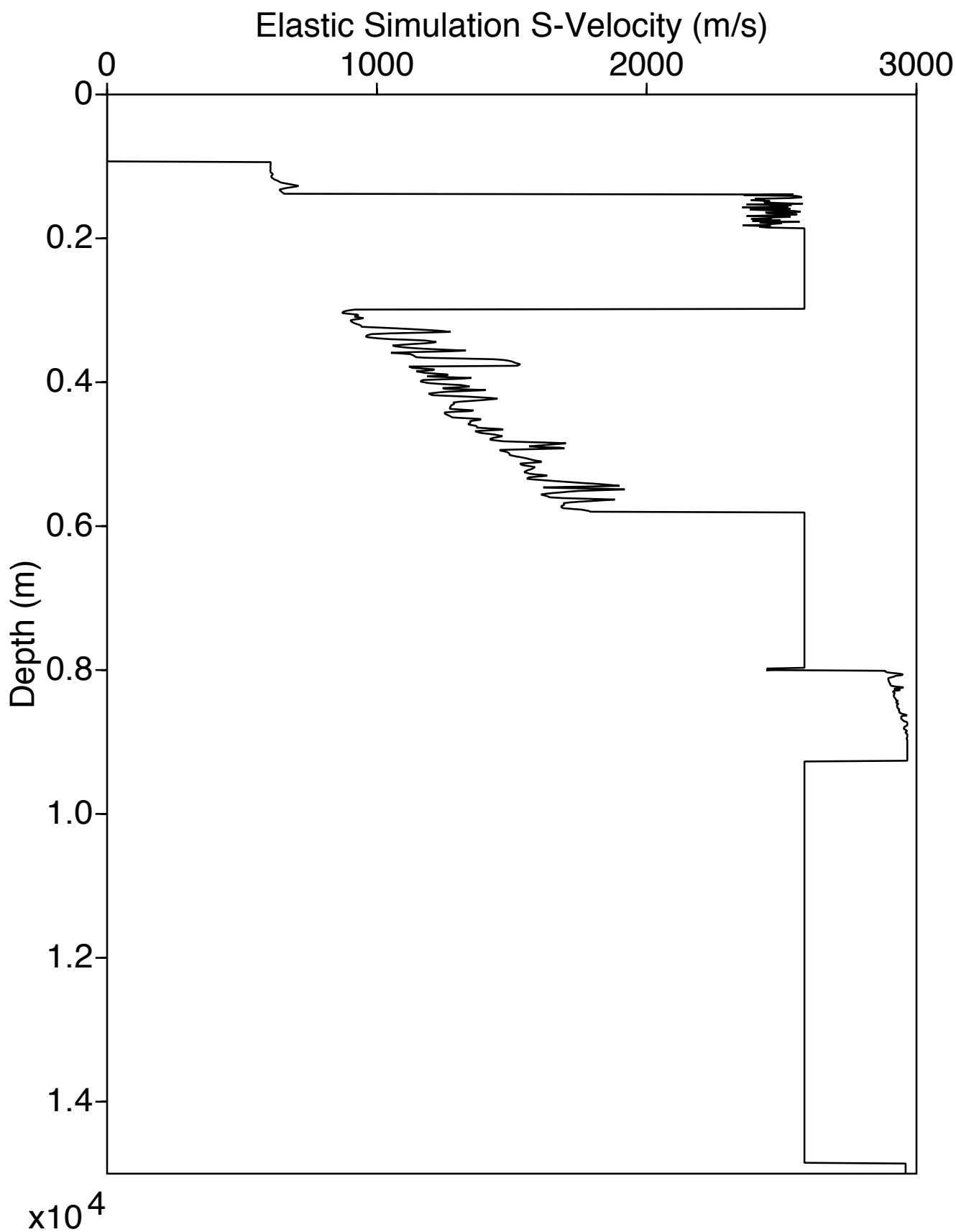
VsElasticSim Log for Well 3
