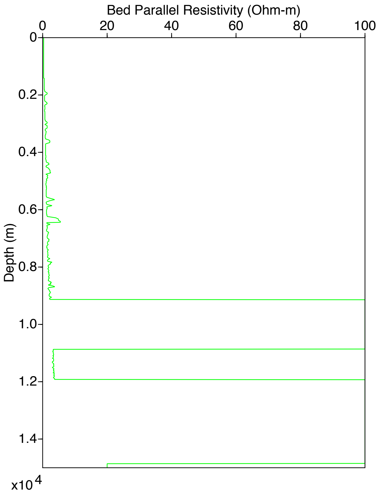
ResistivityParallel Log for Well 1
