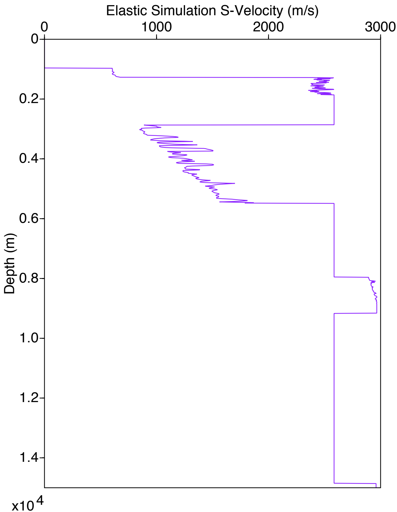
VsElasticSim Log for Well 5
