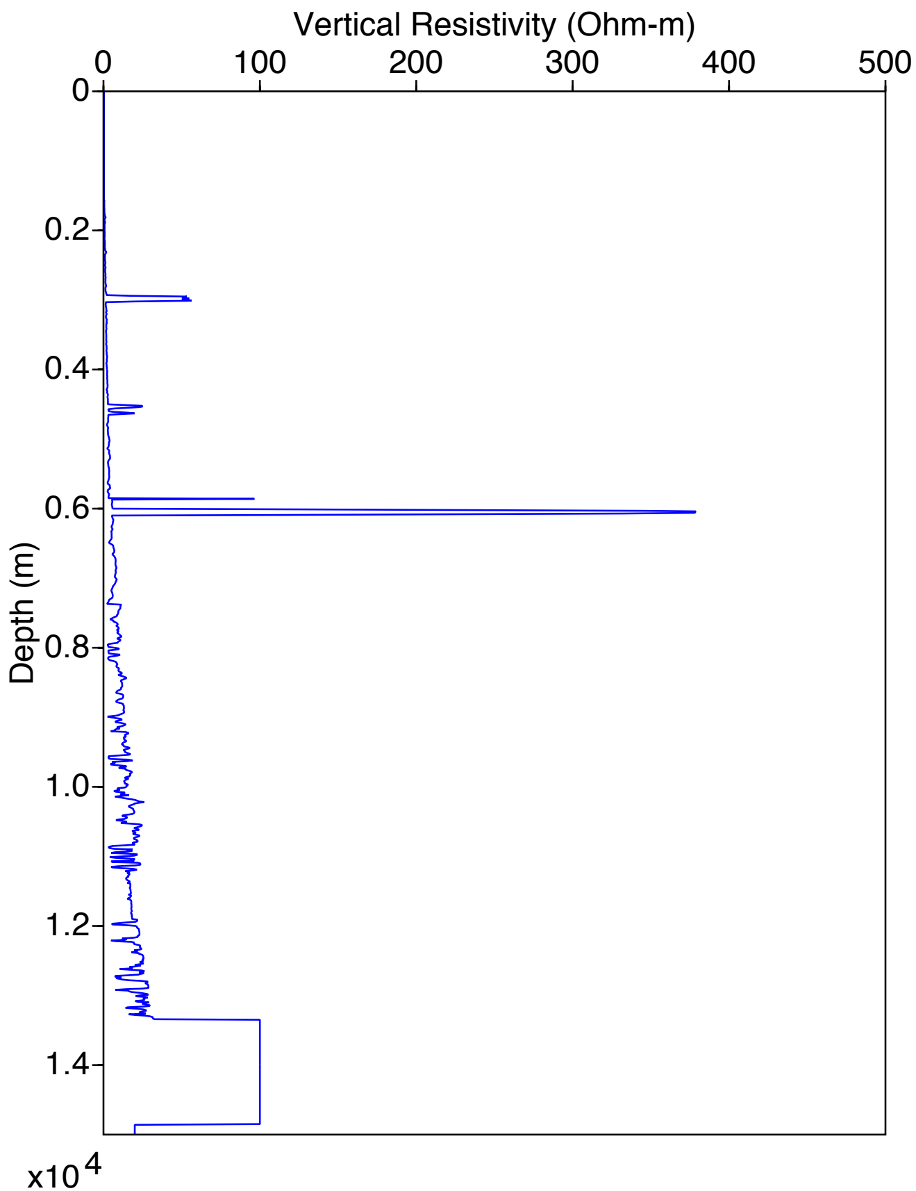
ResistivityVertical Log for Well 4
