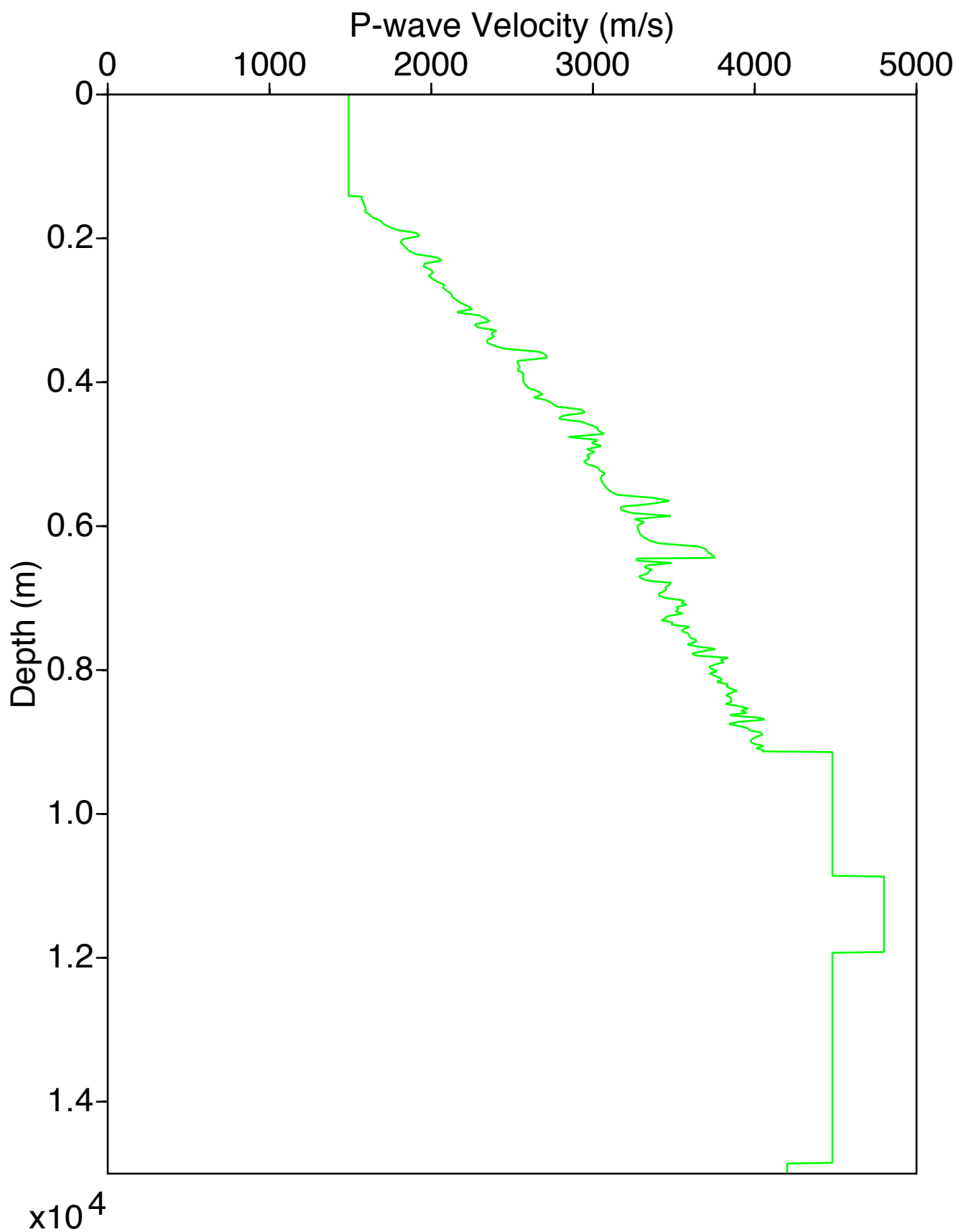
Vp Log for Well 1
