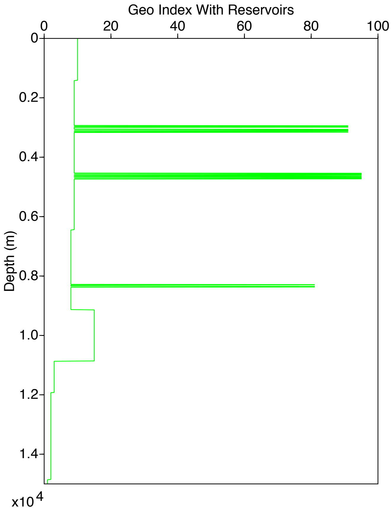
GeoIndexRes Log for Well 1
