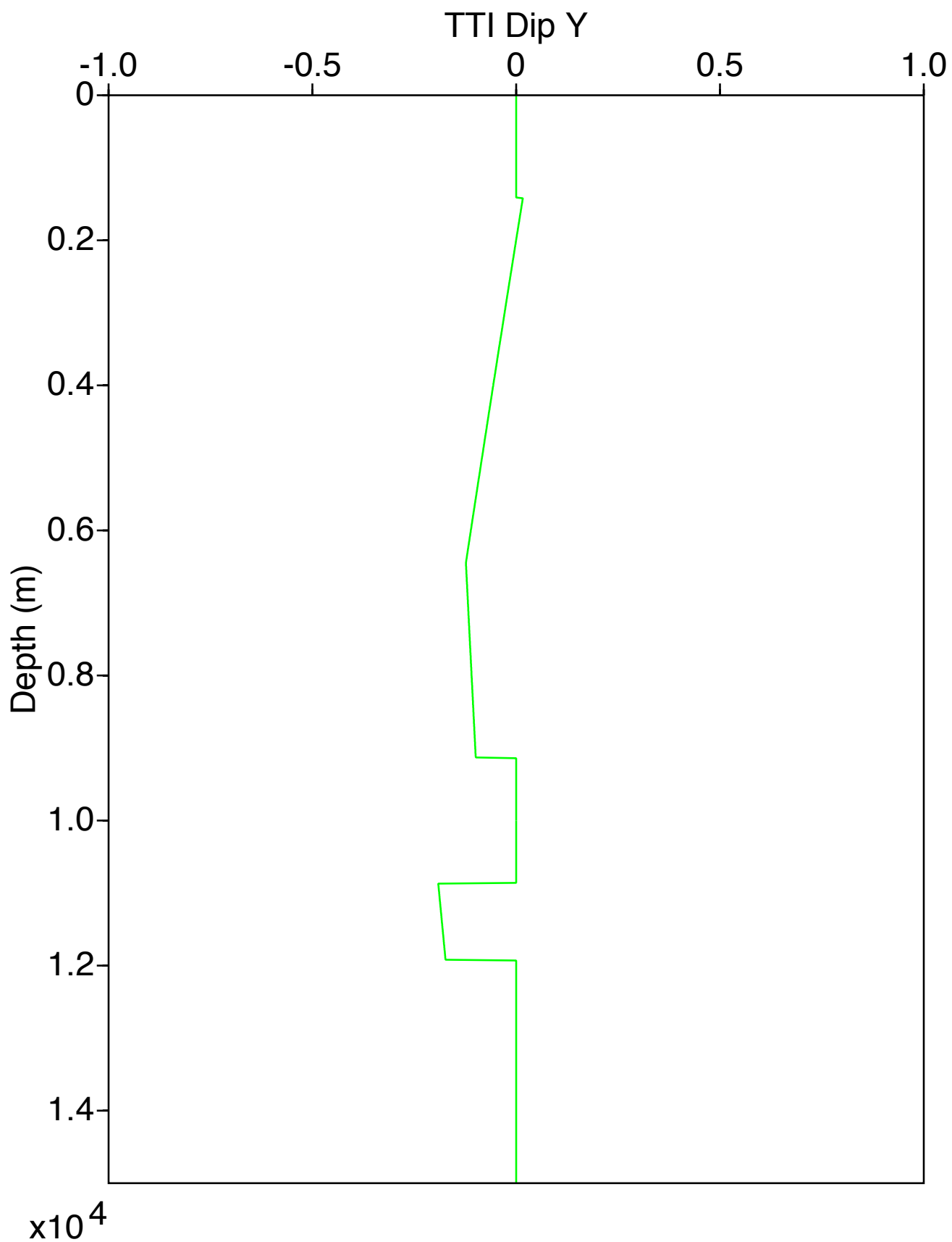
TTIDipY Log for Well 1
