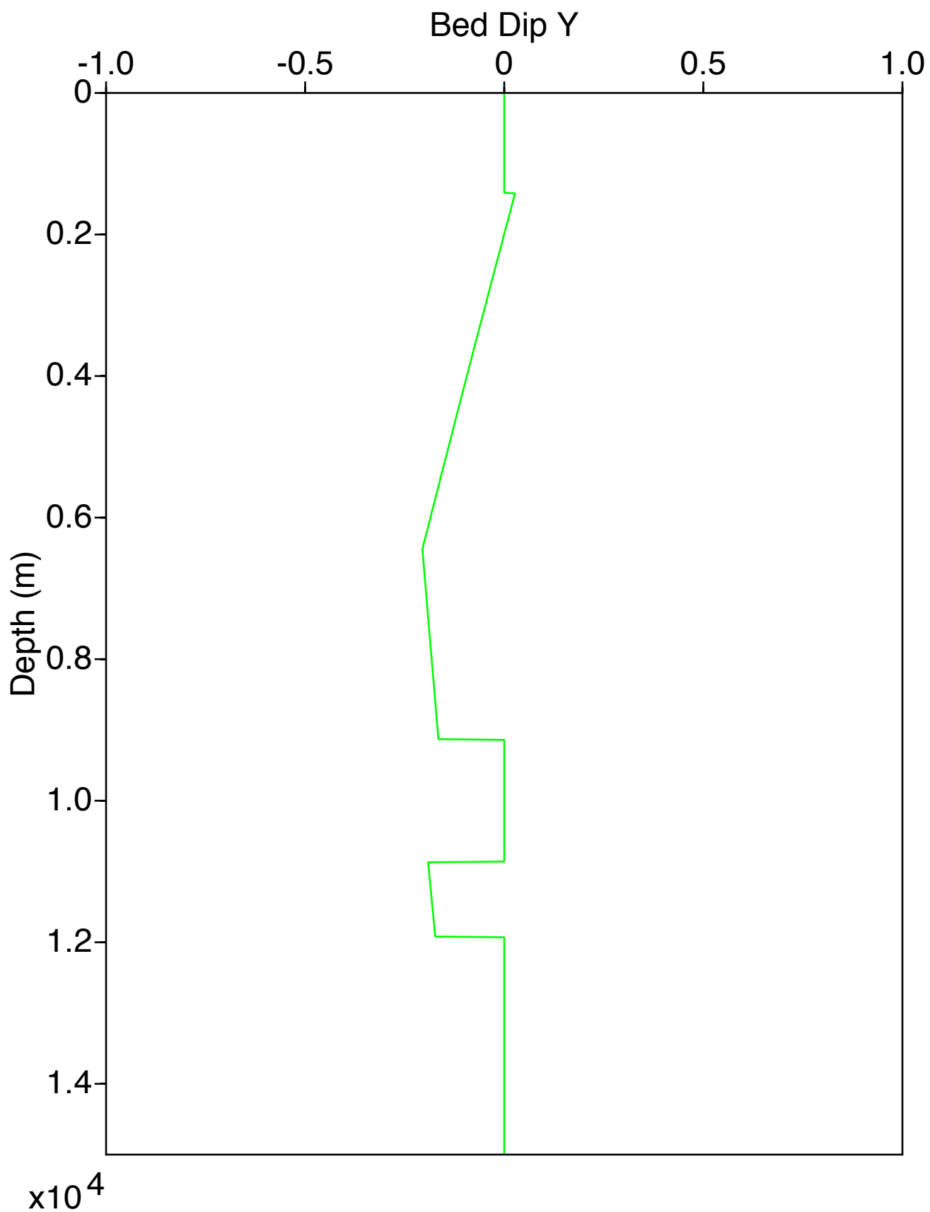
BedDipY Log for Well 1
