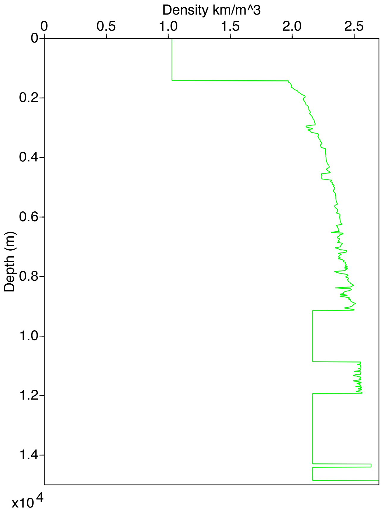
Density Log for Well 1
