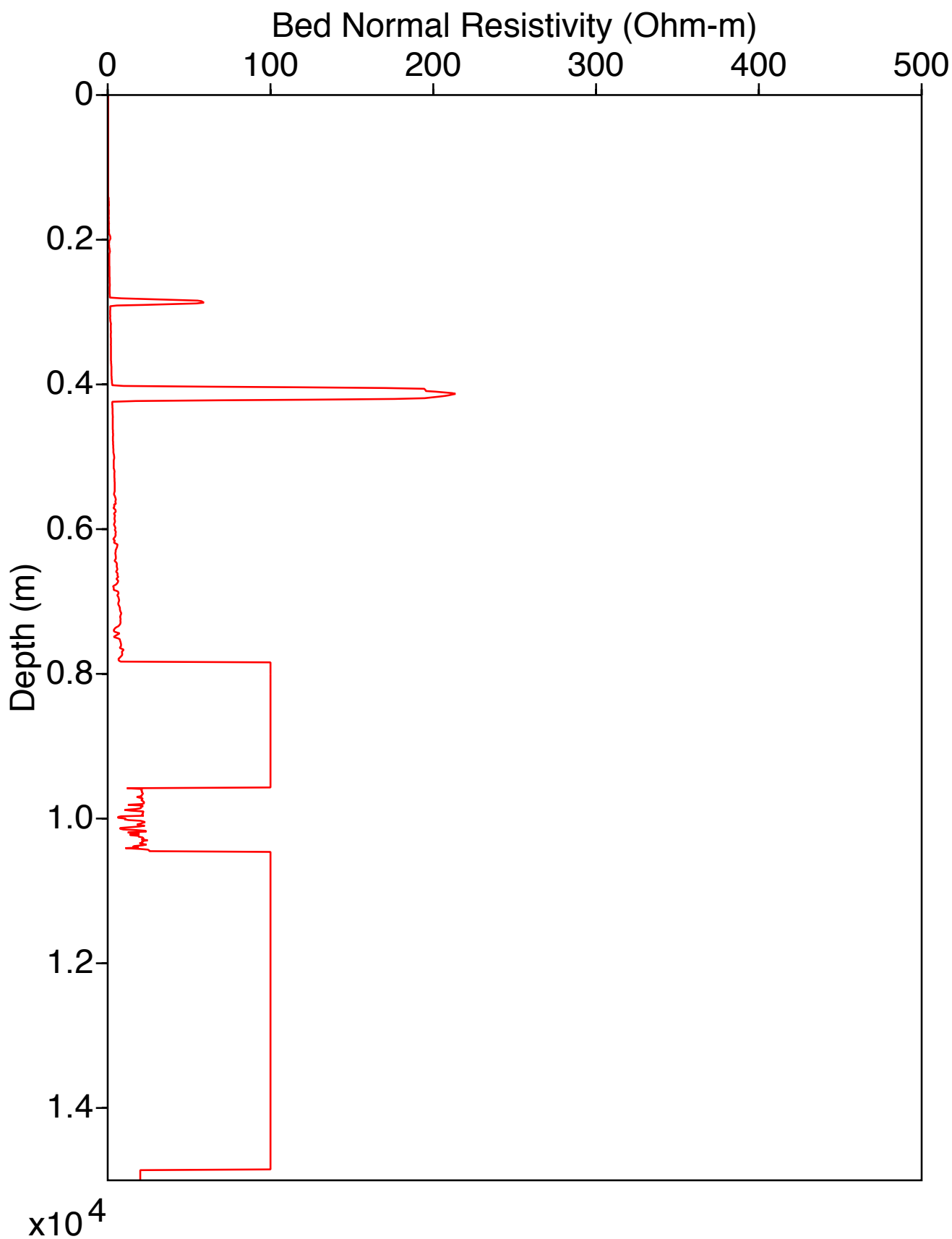
Resistivity Normal Log for Well 2
