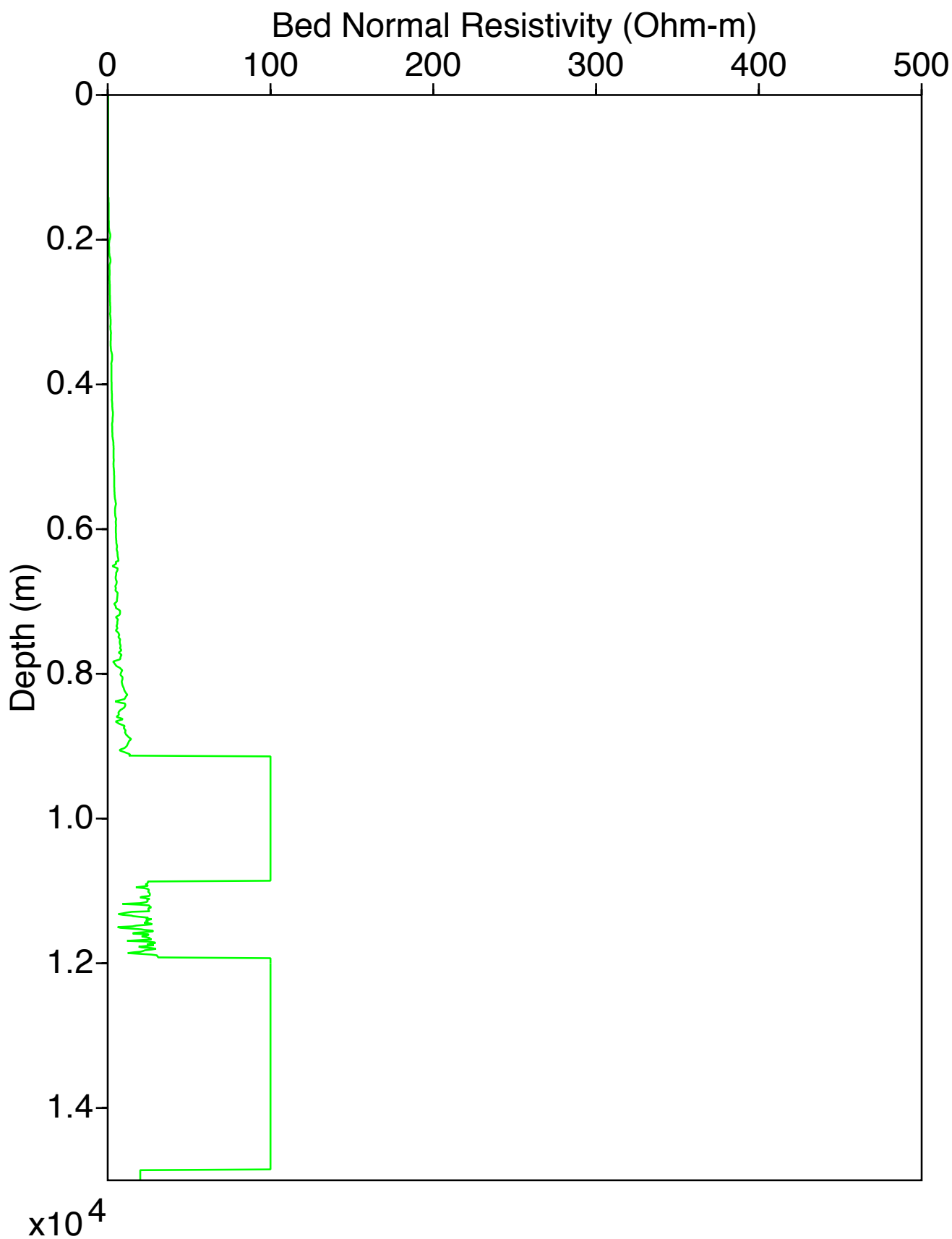
Resistivity Normal Log for Well 1
