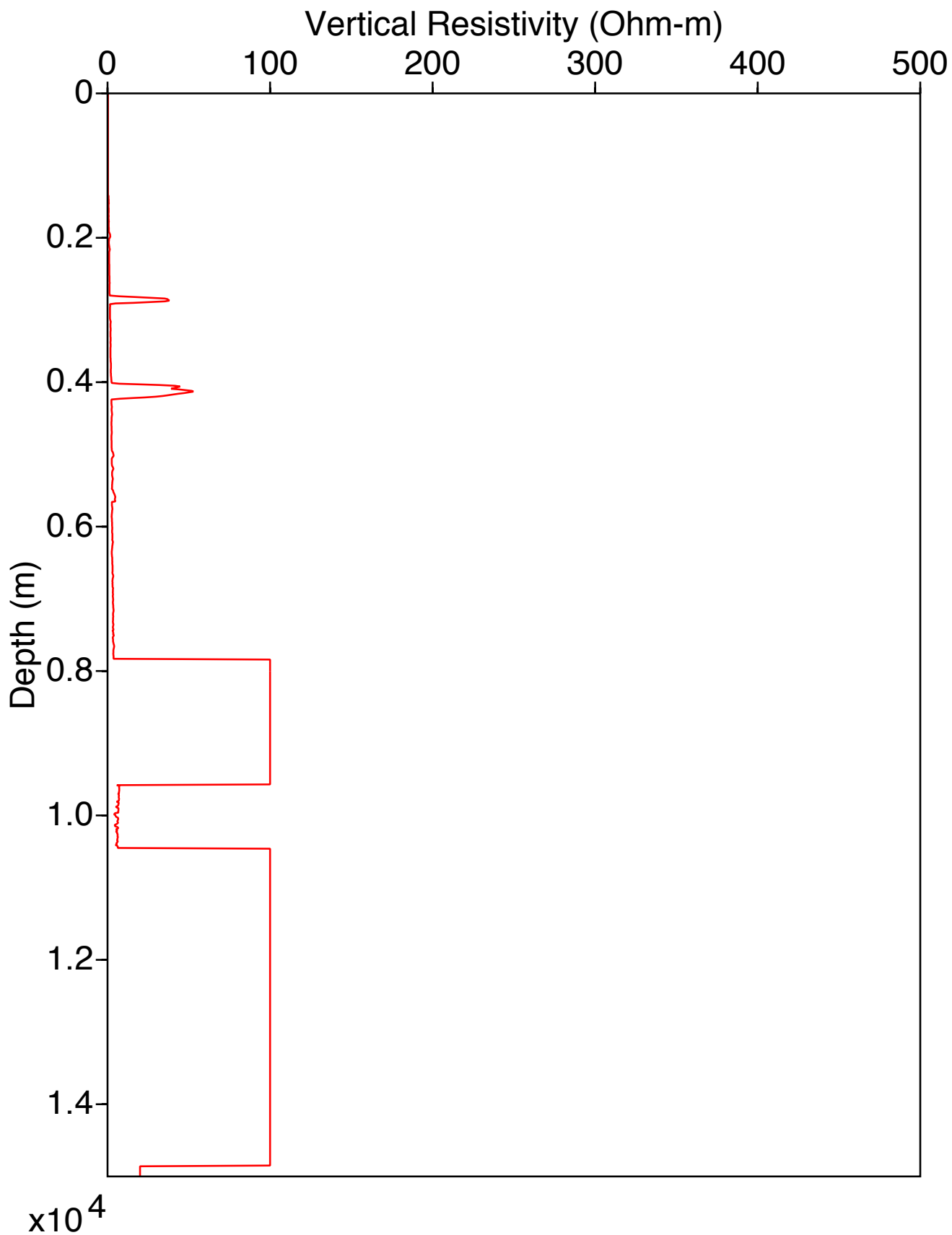
Resistivity Vertical Log for Well 2
