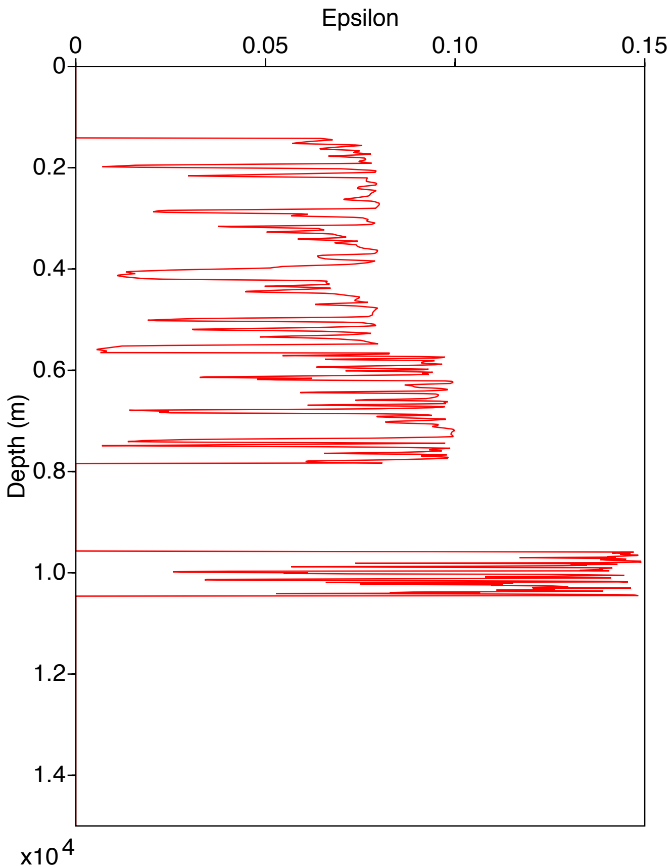
Epsilon Log for Well 2
