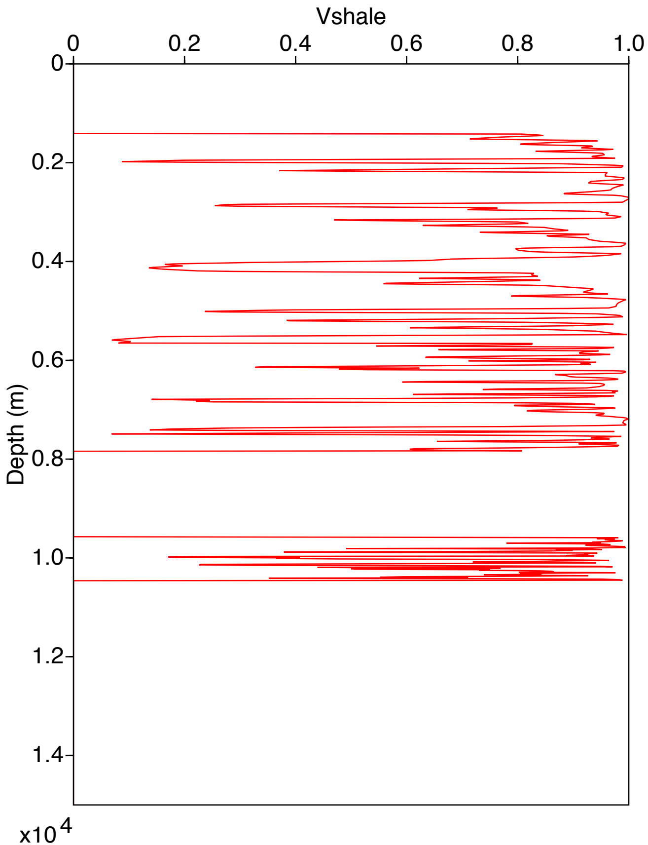
Vshale Log for Well 2
