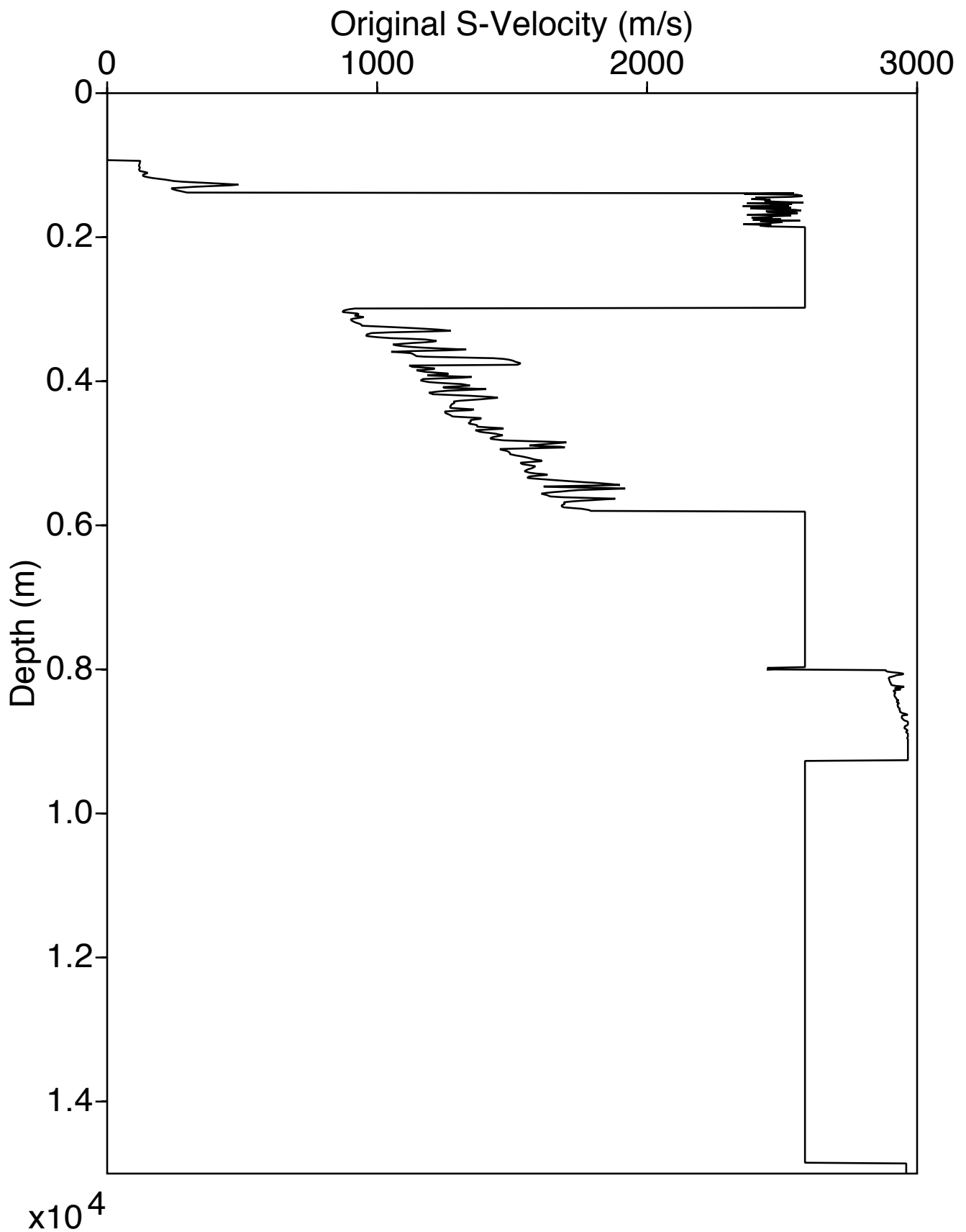
VsElasticOriginal Log for Well 3
