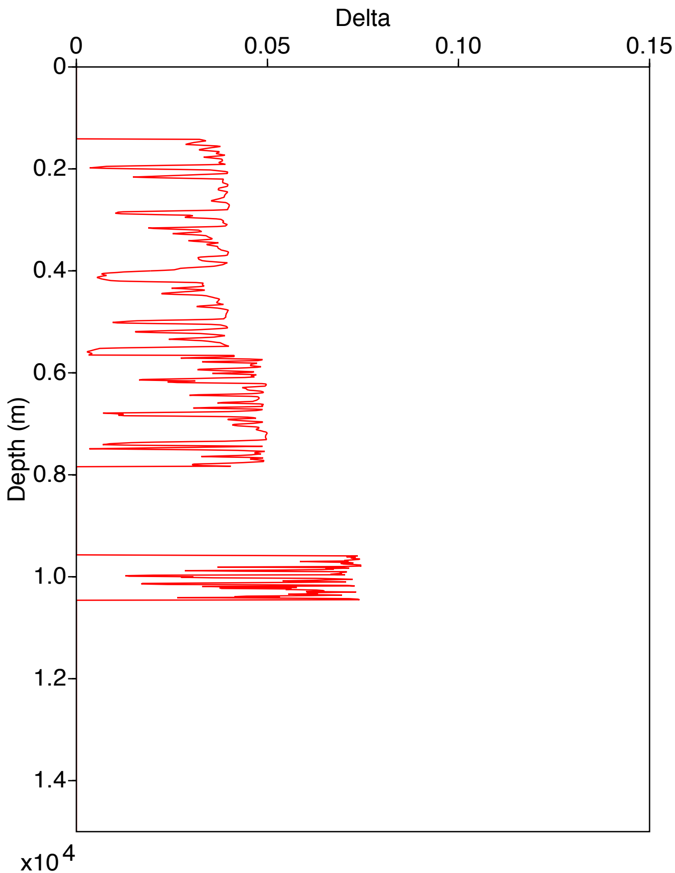
Delta Log for Well 2
