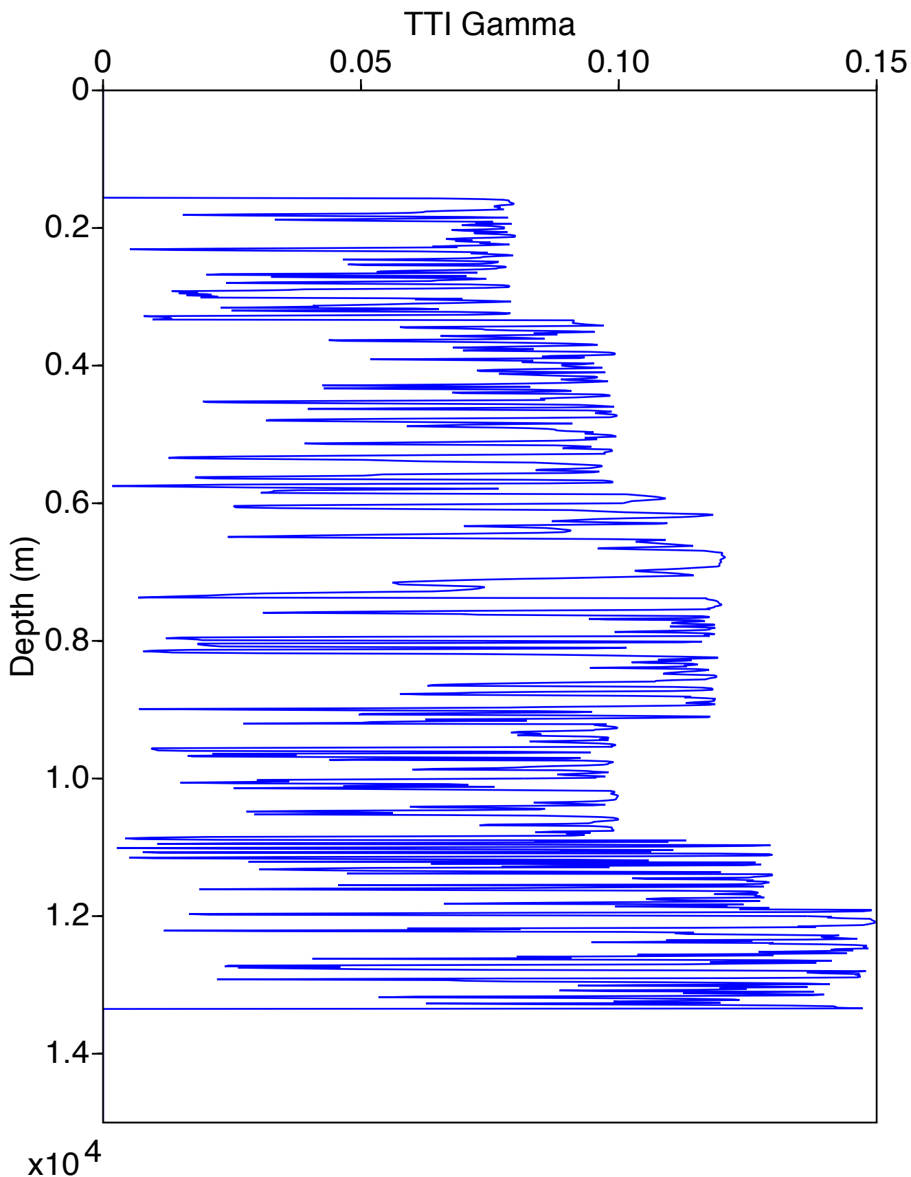
Gamma Log for Well 4
