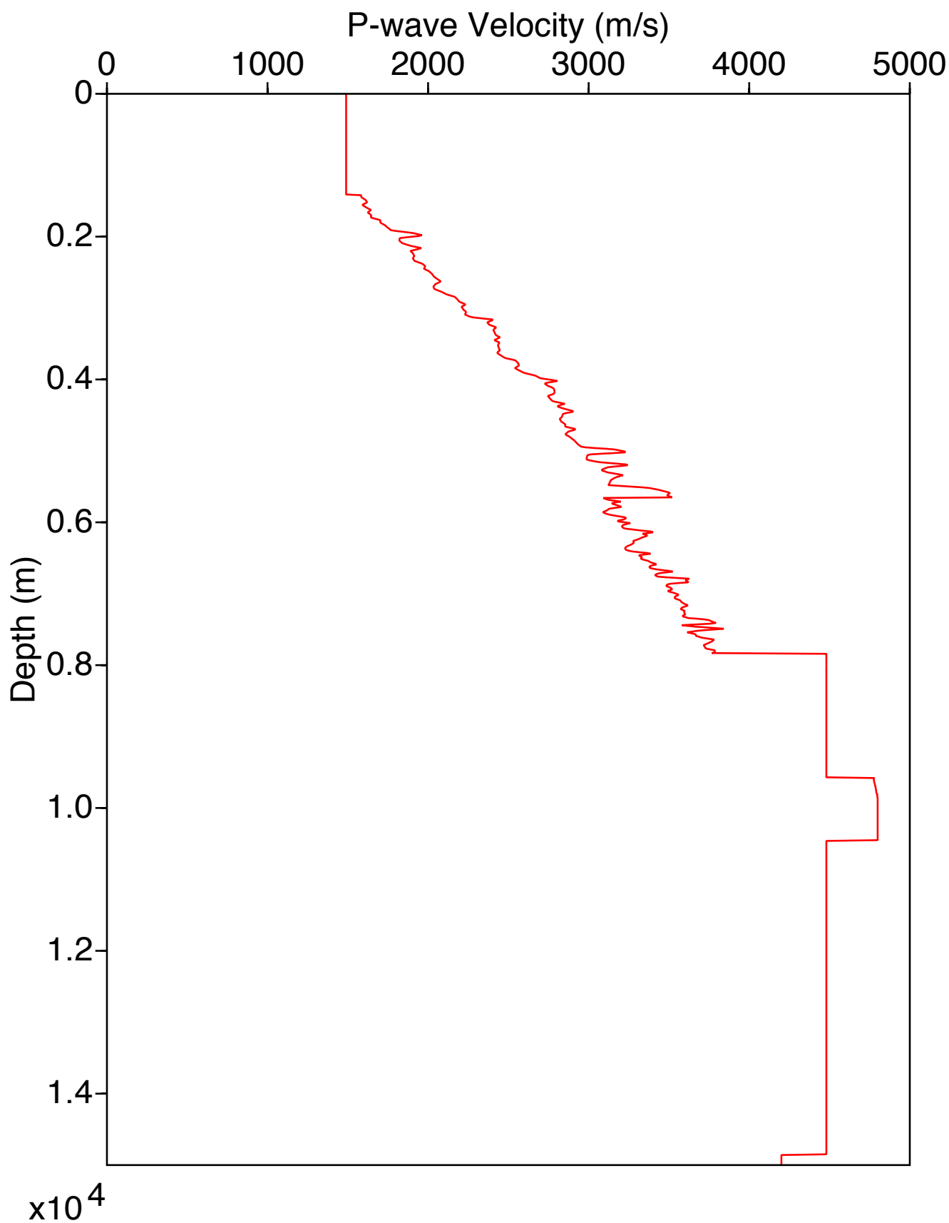
Vp Log for Well 2
