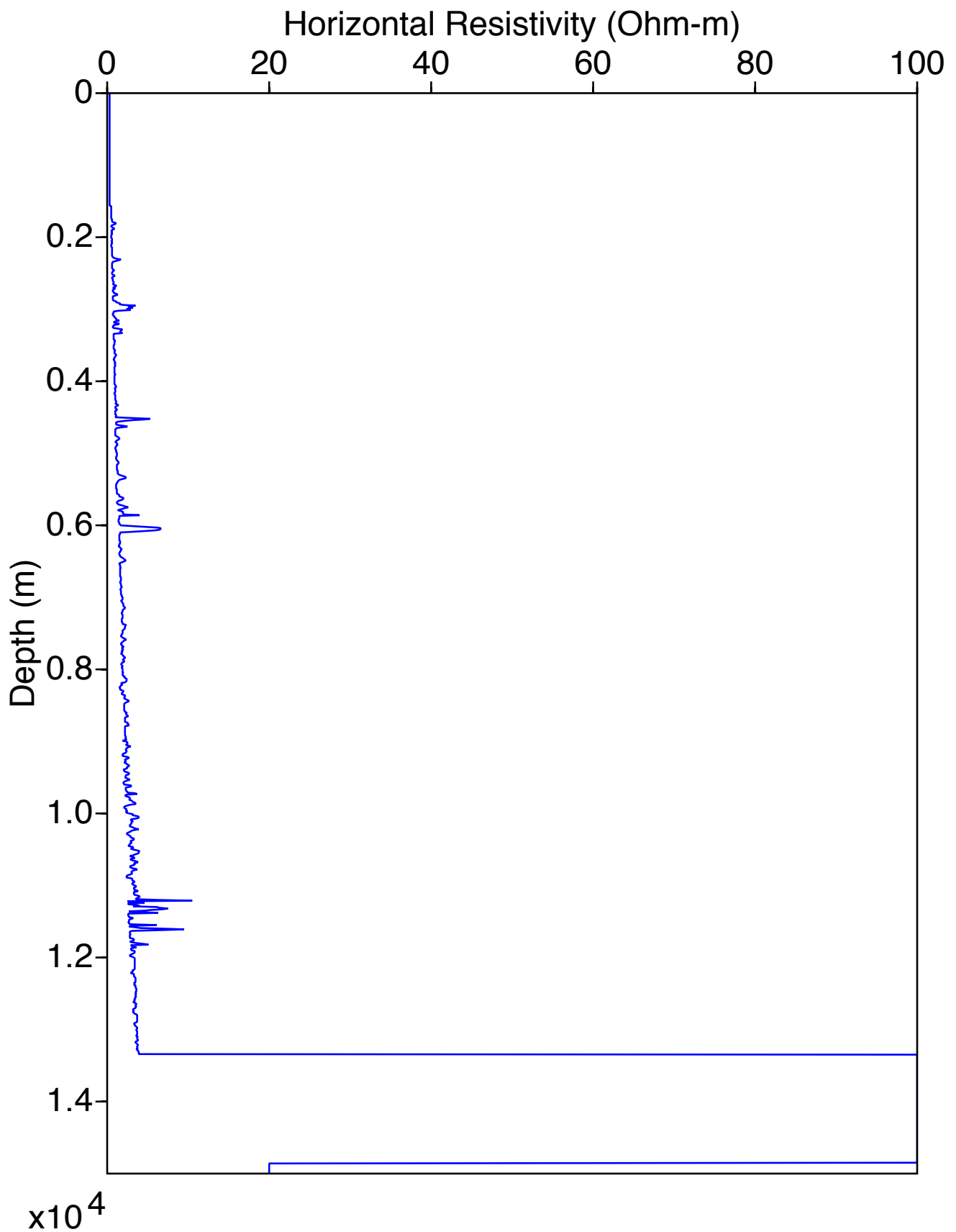
ResistivityHorizontal Log for Well 4
