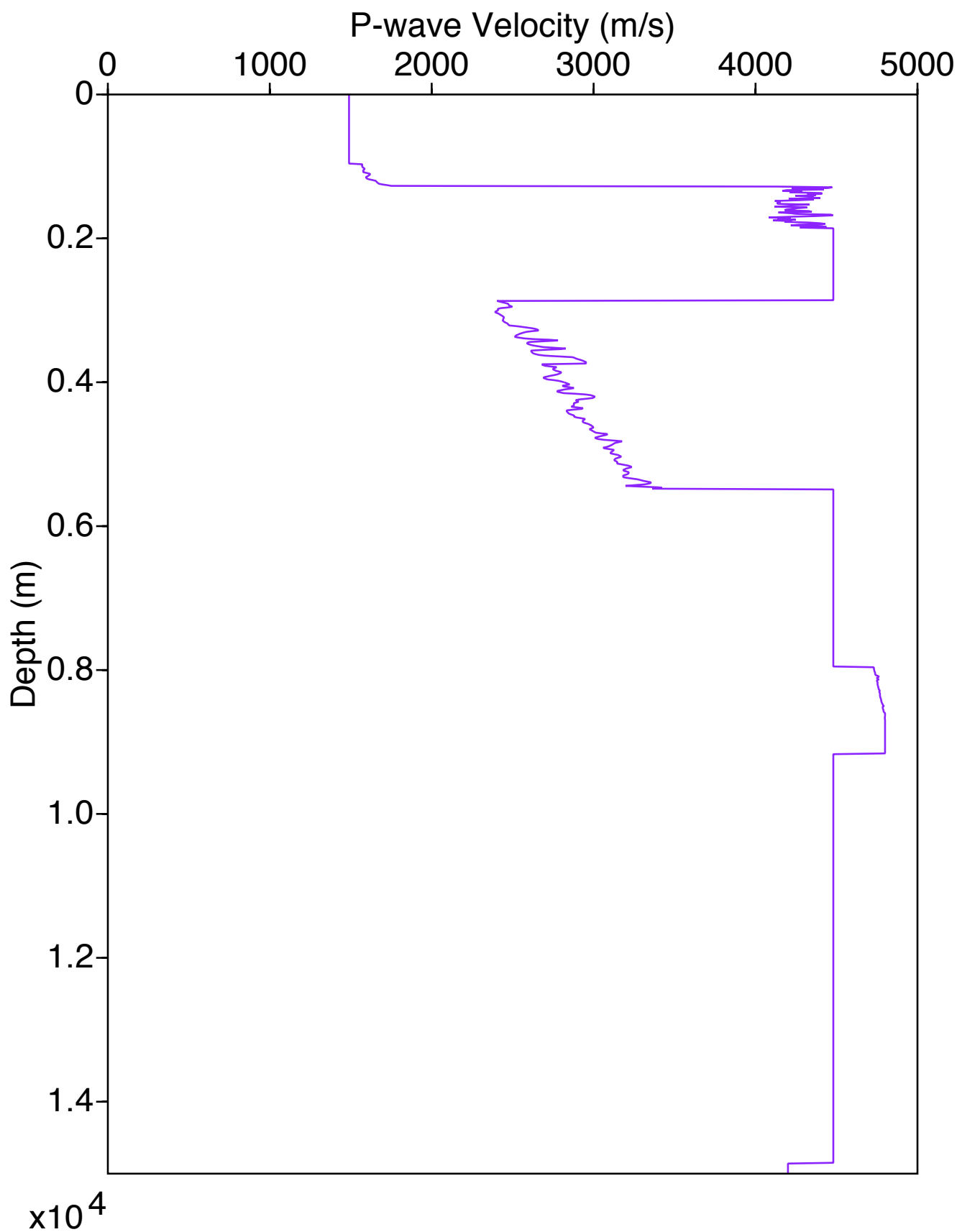
Vp Log for Well 5
