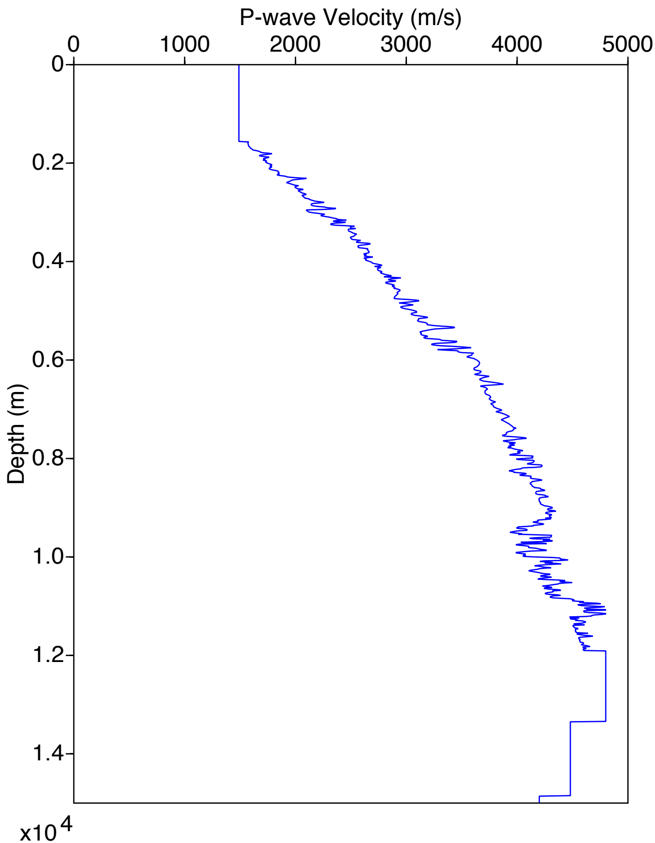
Vp Log for Well 4
