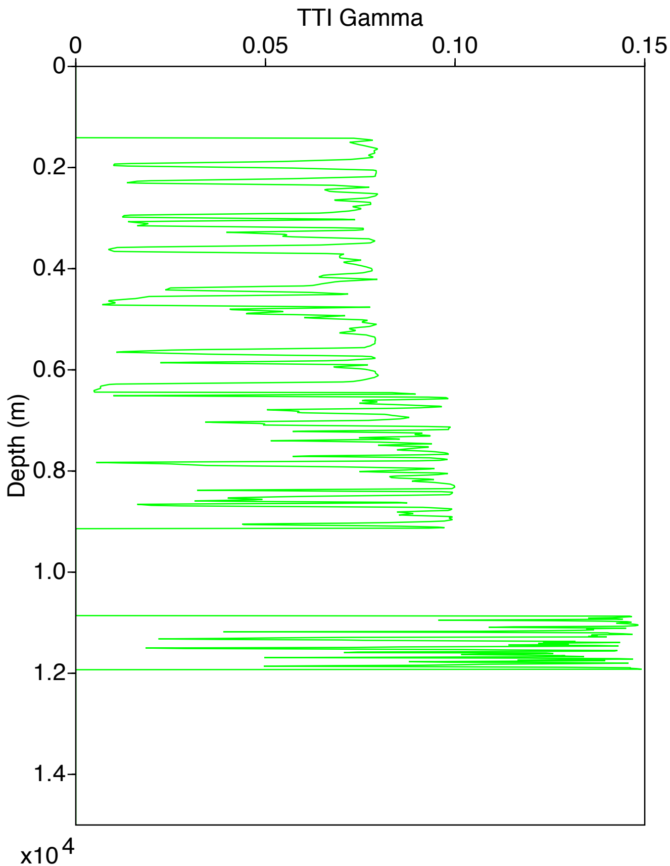
Gamma Log for Well 1
