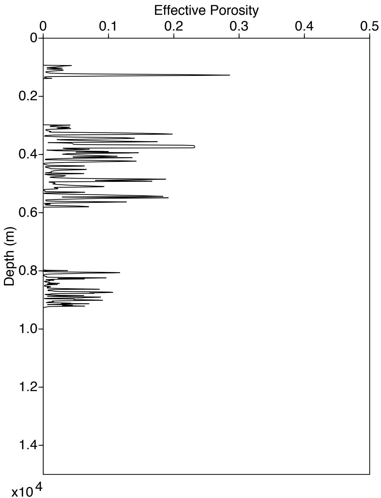
PorosityEffective Log for Well 3
