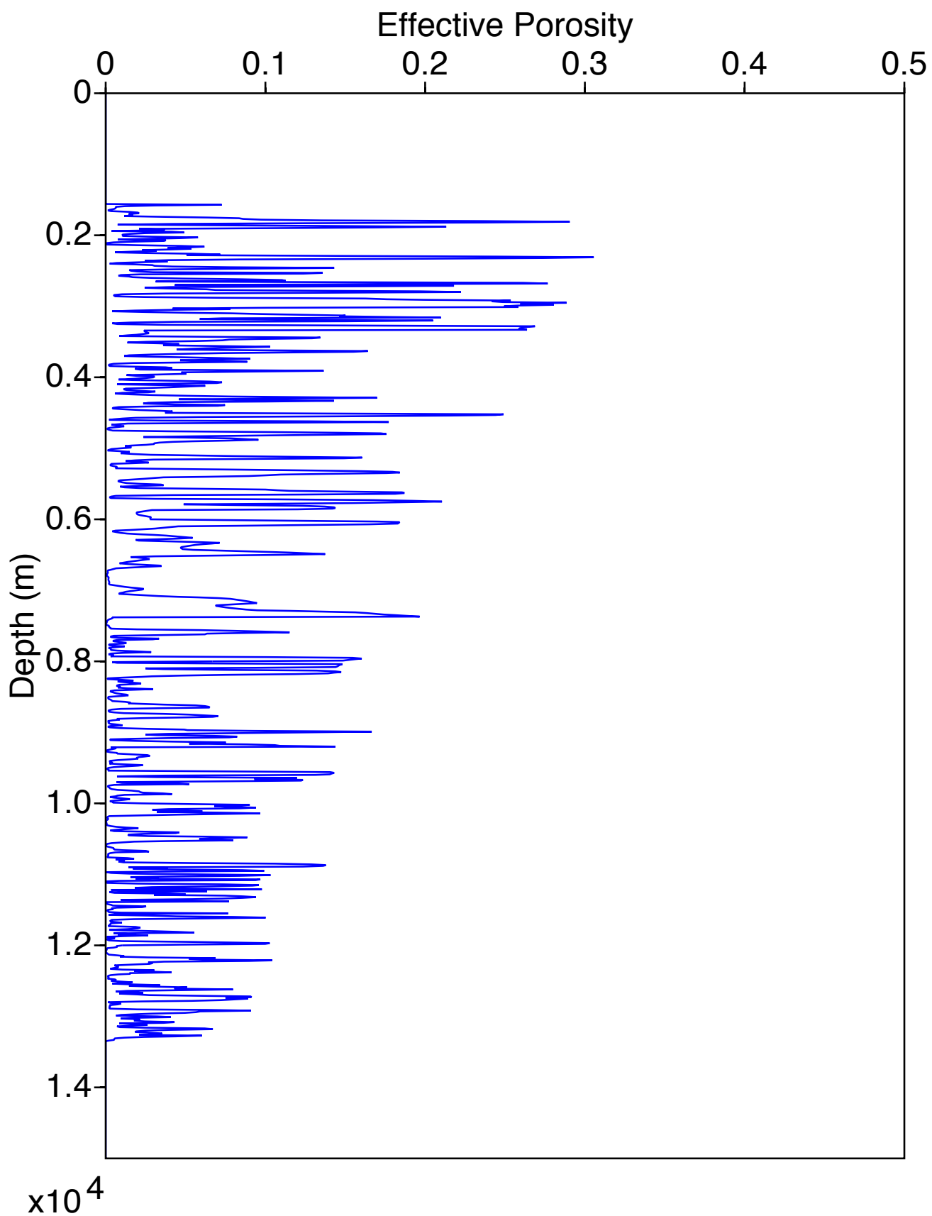
PorosityEffective Log for Well 4
