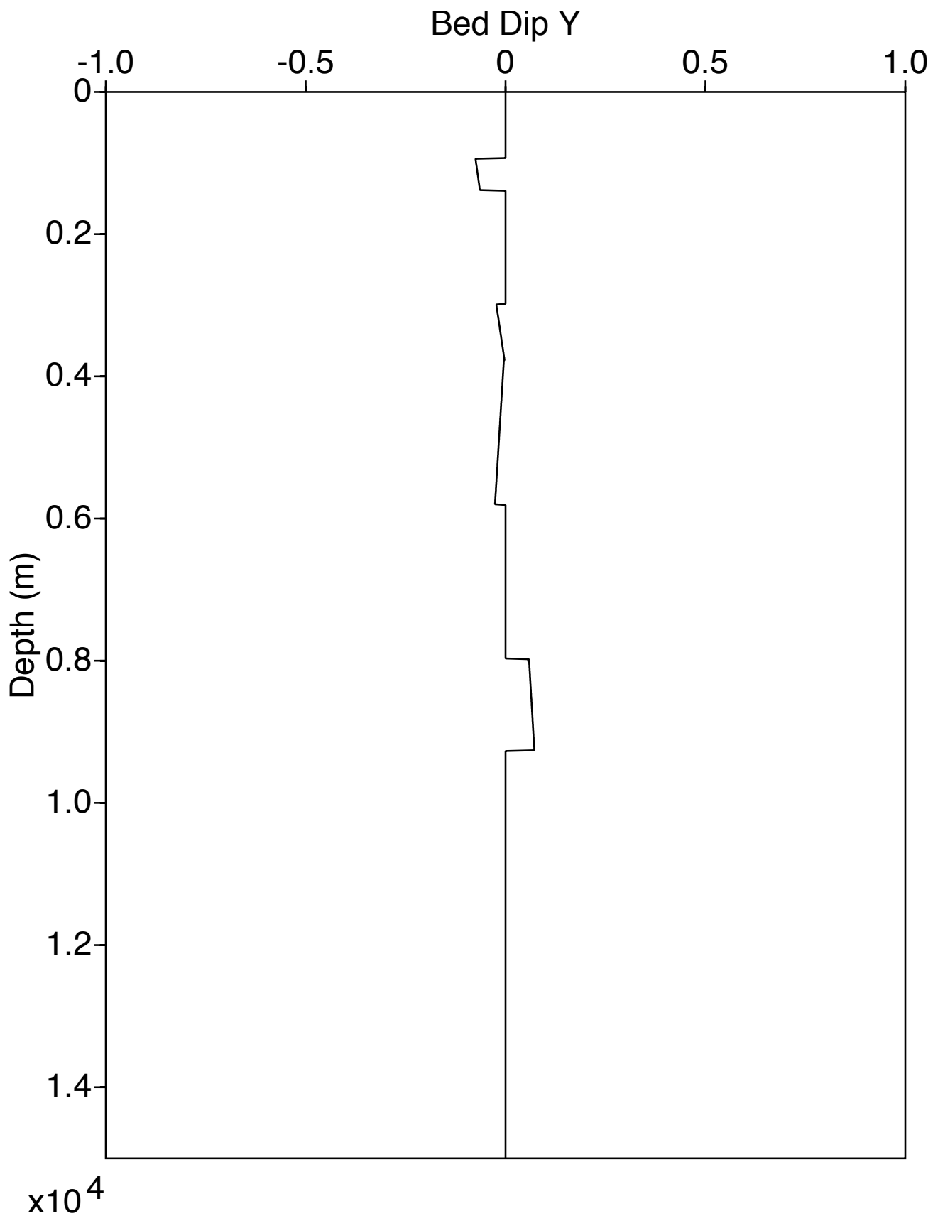
BedDipY Log for Well 3
