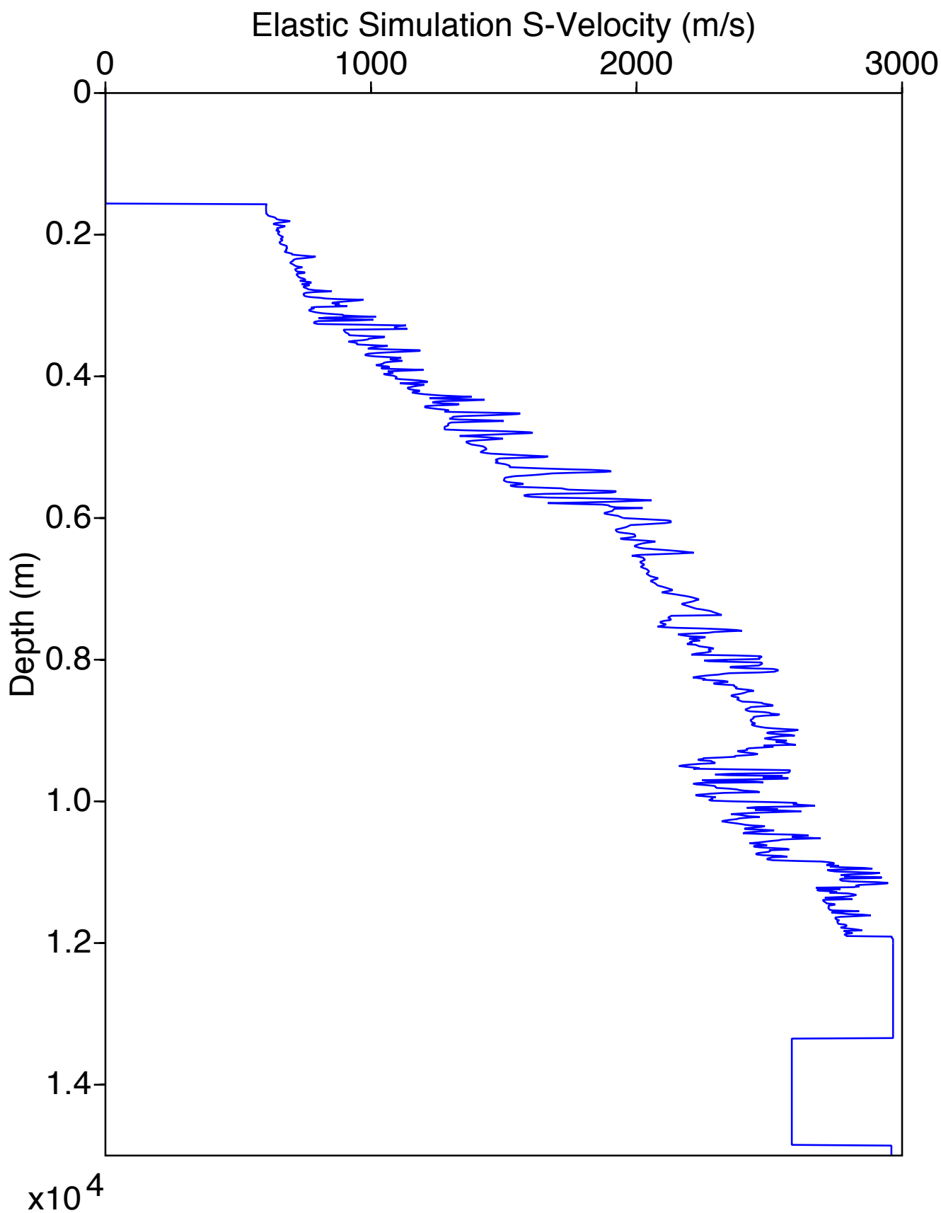
VsElasticSim Log for Well 4
