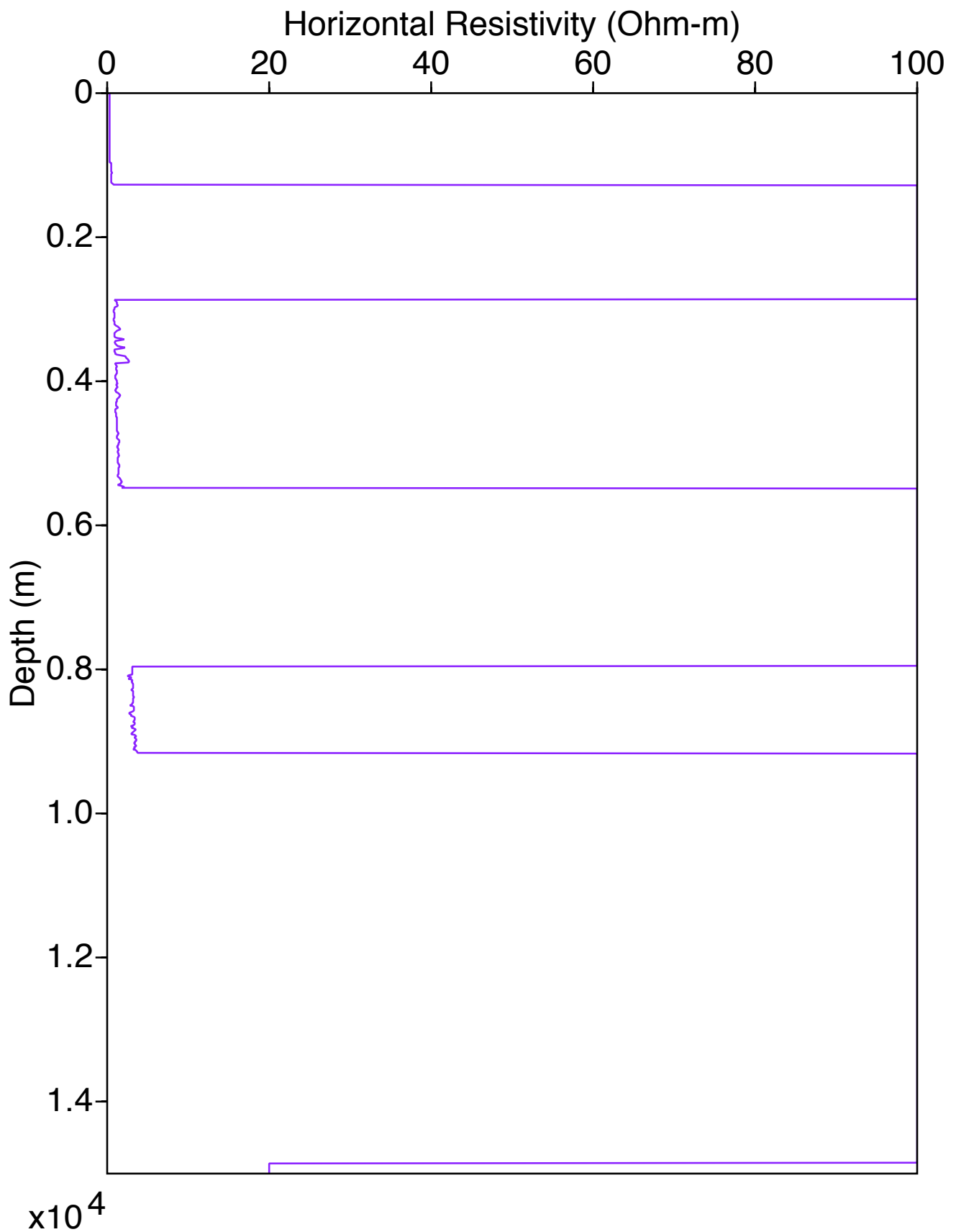
ResistivityHorizontal Log for Well 5
