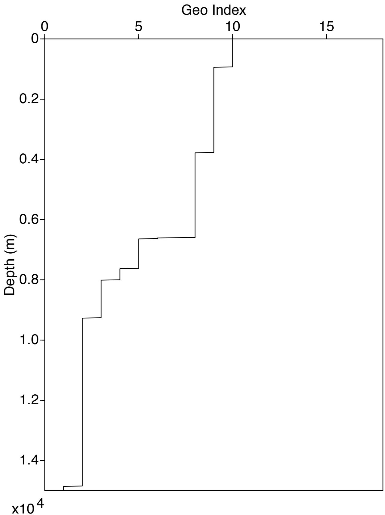
LayerGeoIndex Log for Well 3
