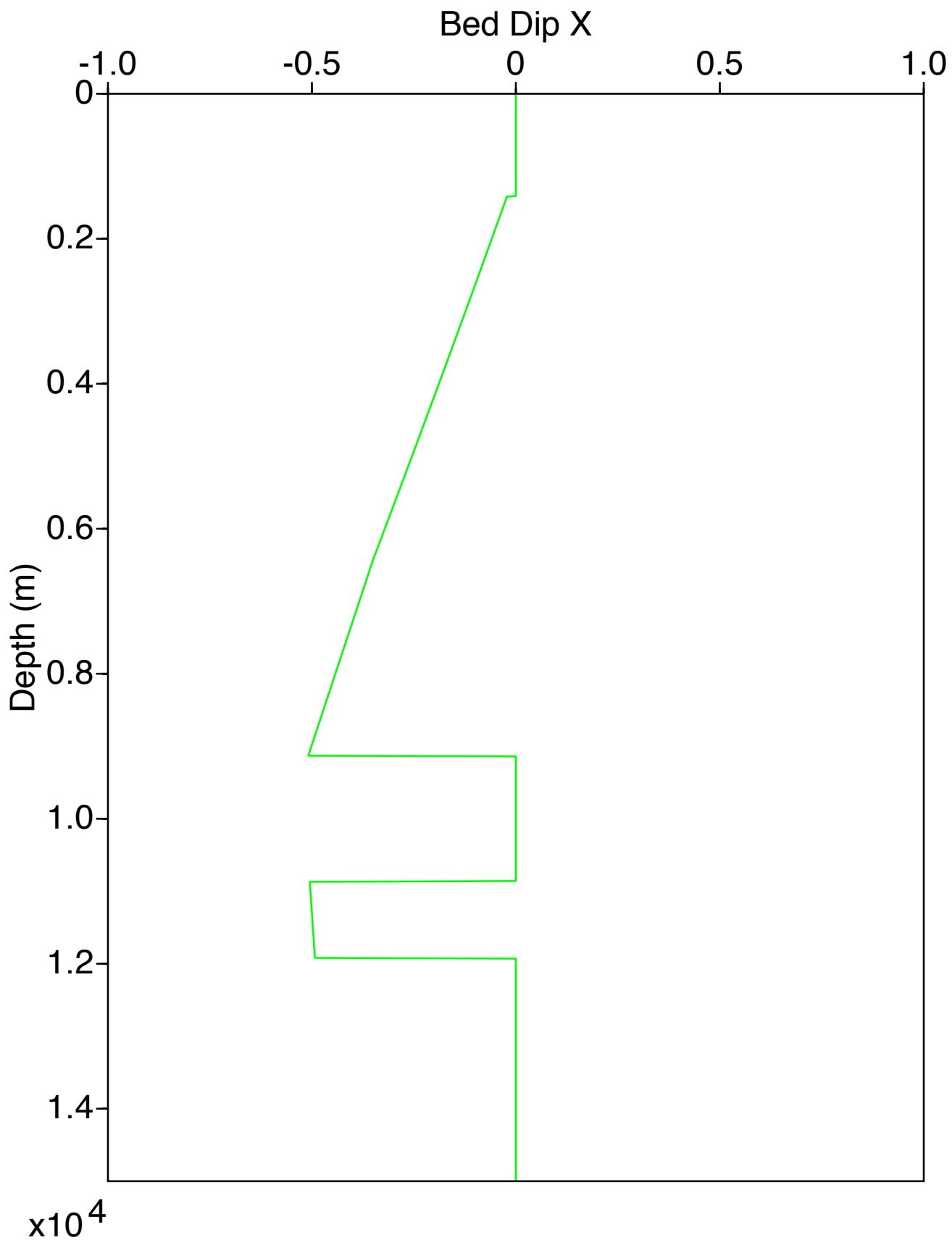
BedDipX Log for Well 1
