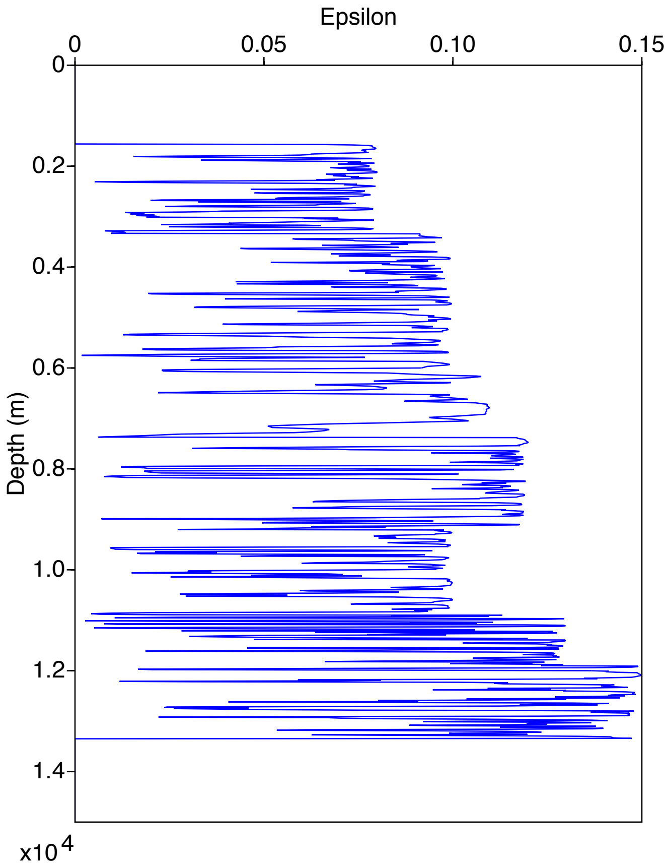
Epsilon Log for Well 4
