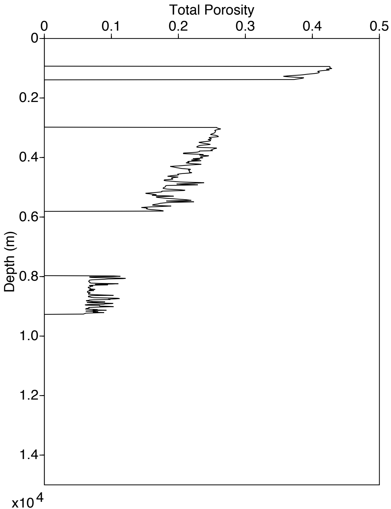
PorosityTotal Log for Well 3
