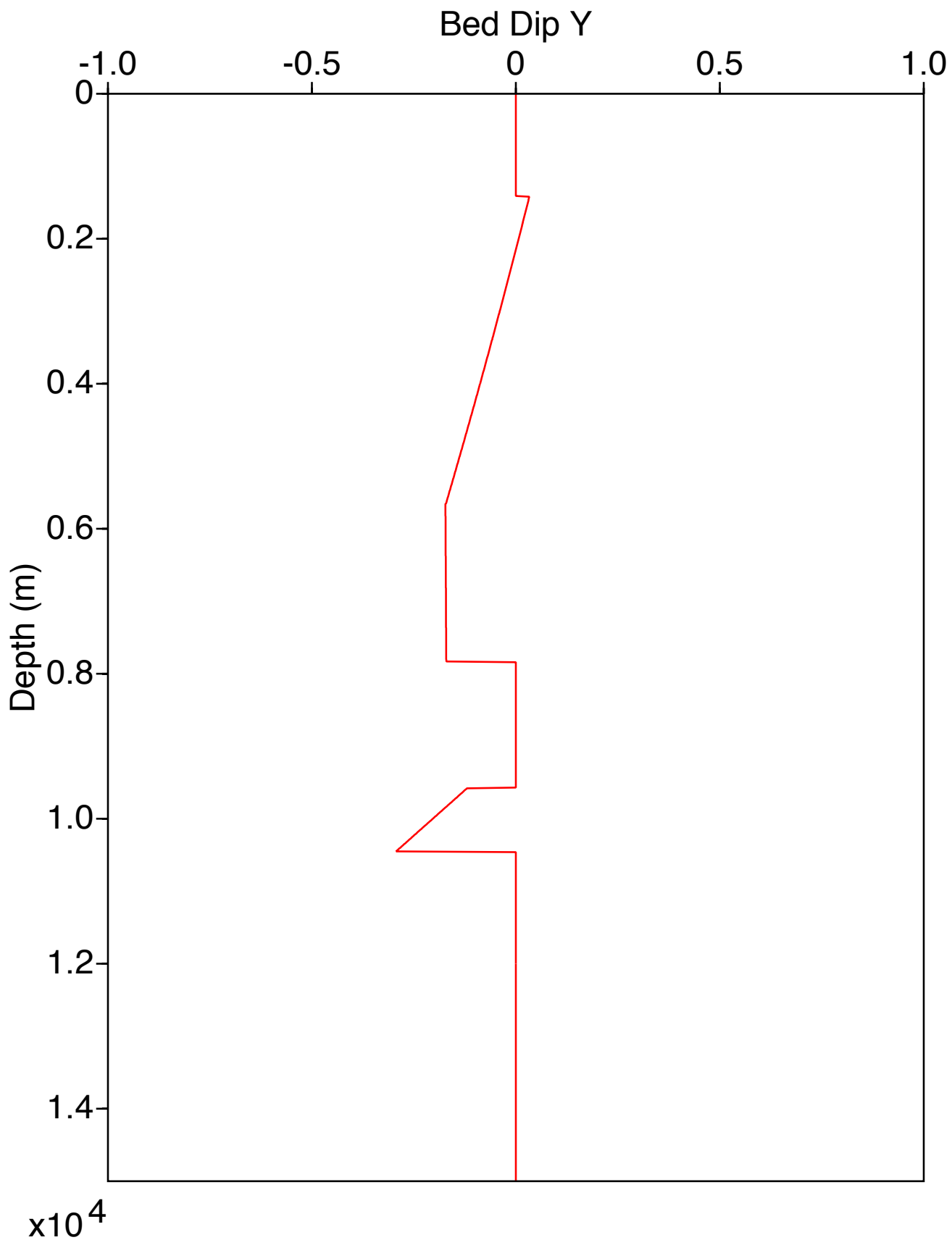
BedDipY Log for Well 2
