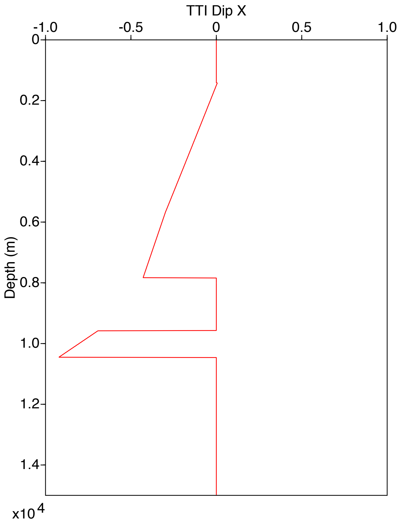
TTIDipX Log for Well 2
