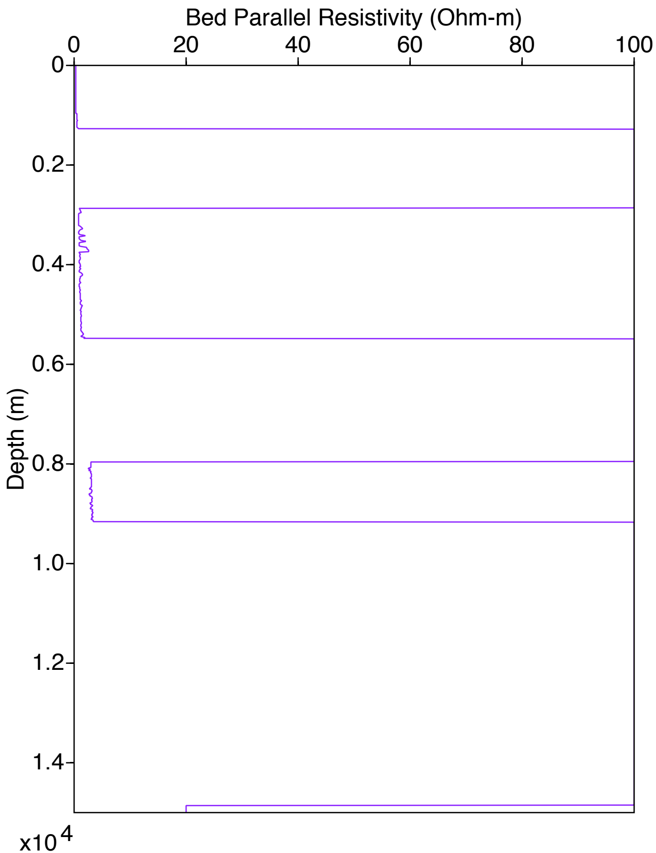
ResistivityParallel Log for Well 5
