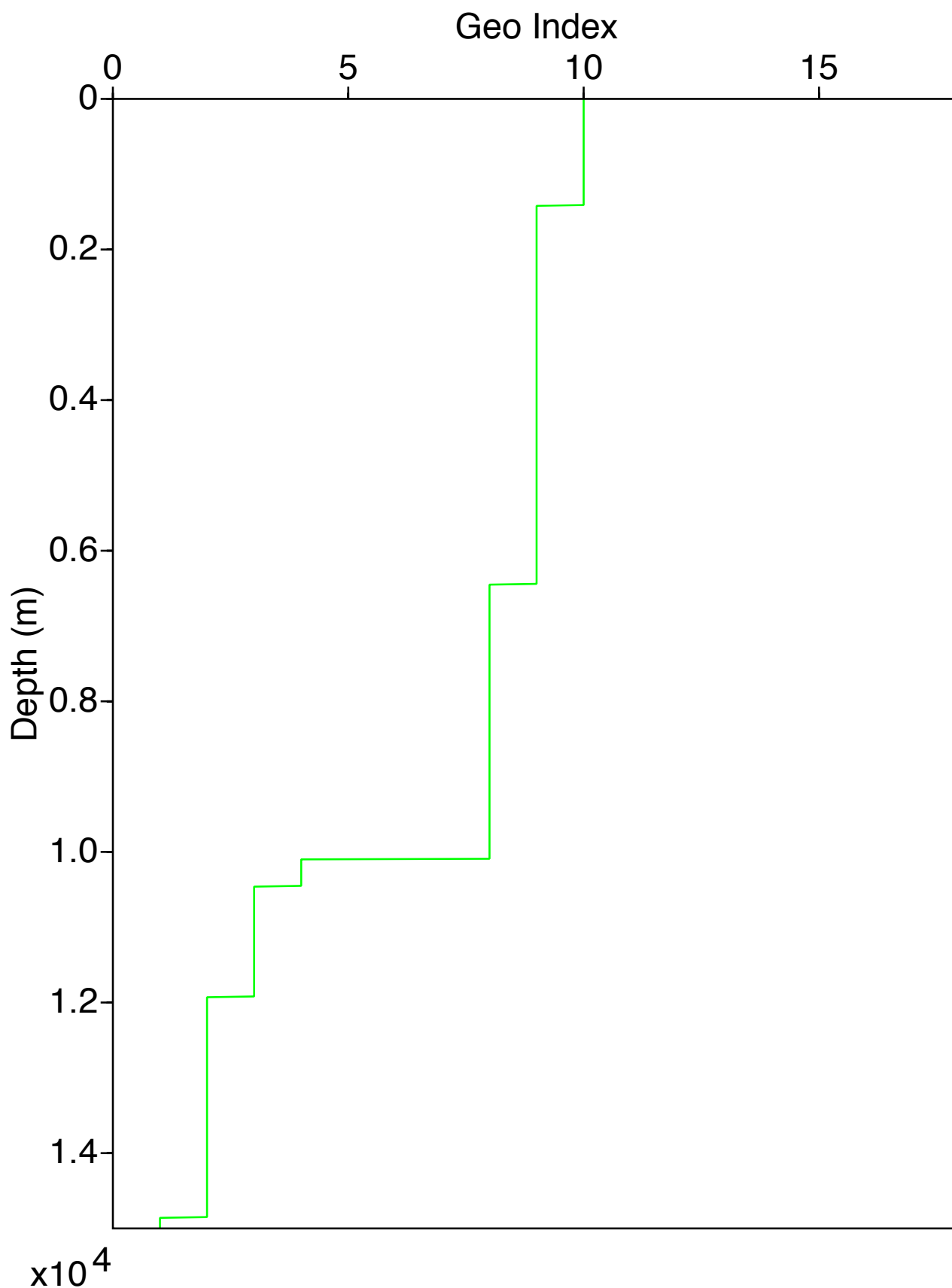
LayerGeoIndex Log for Well 1
