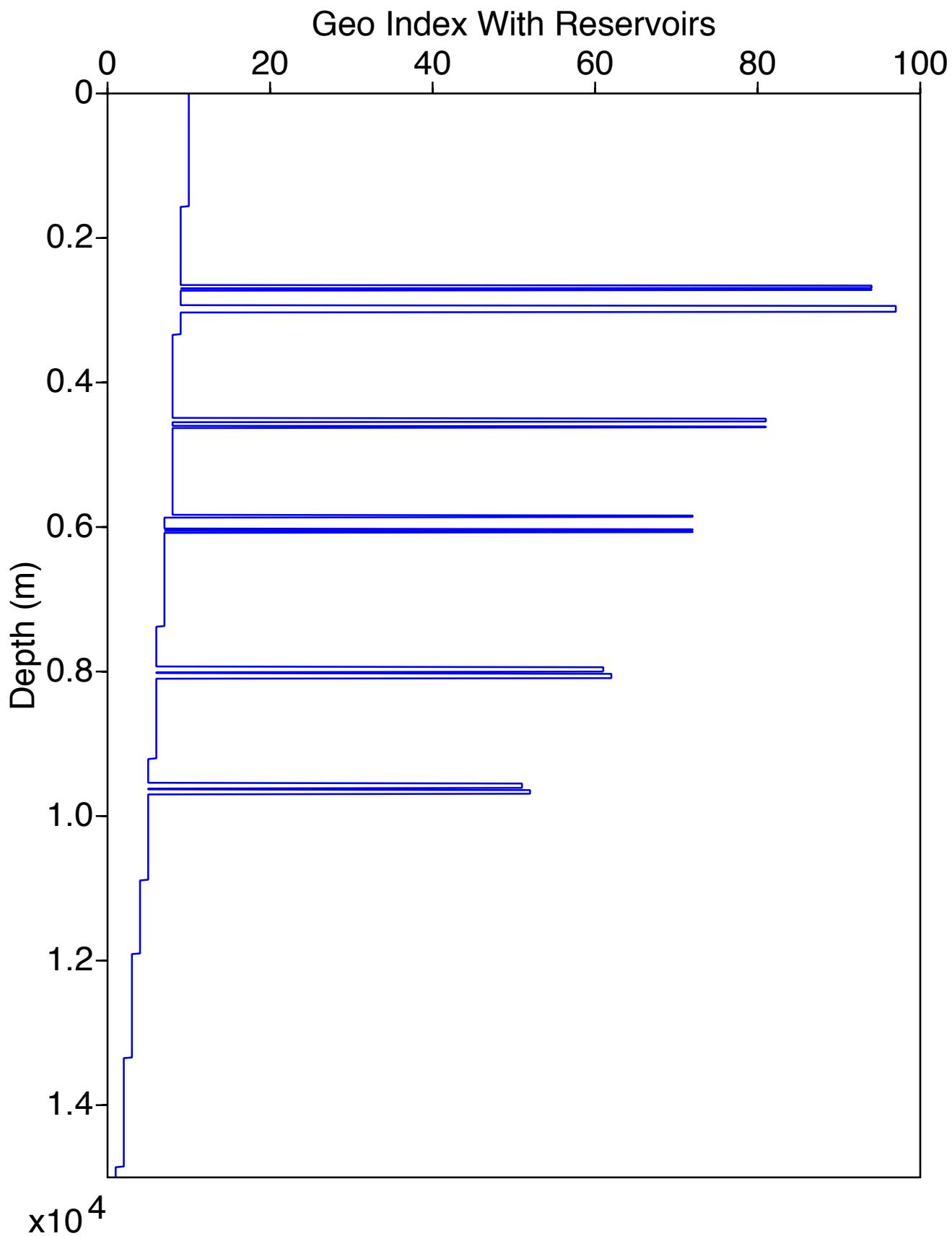
GeoIndexRes Log for Well 4
