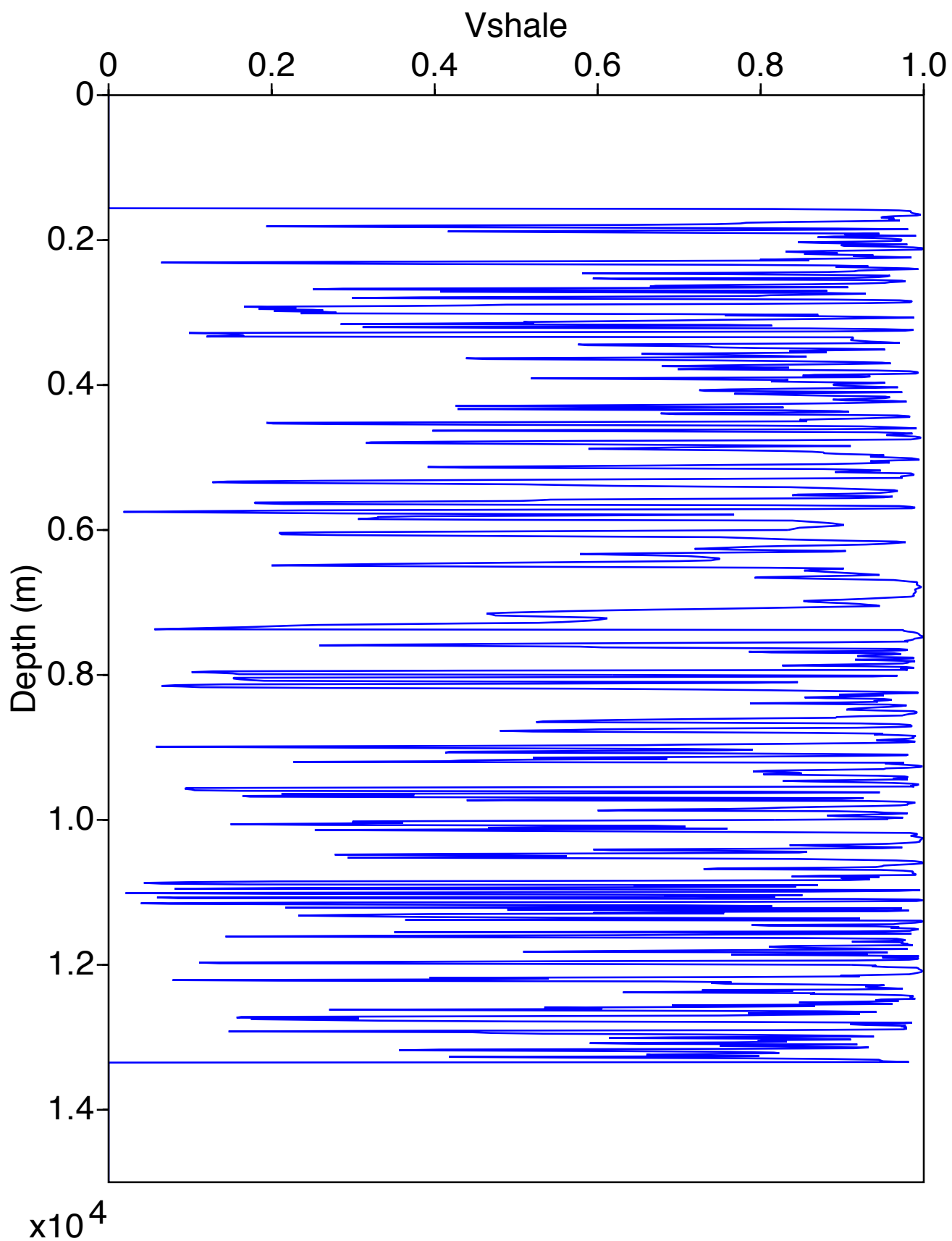
Vshale Log for Well 4
