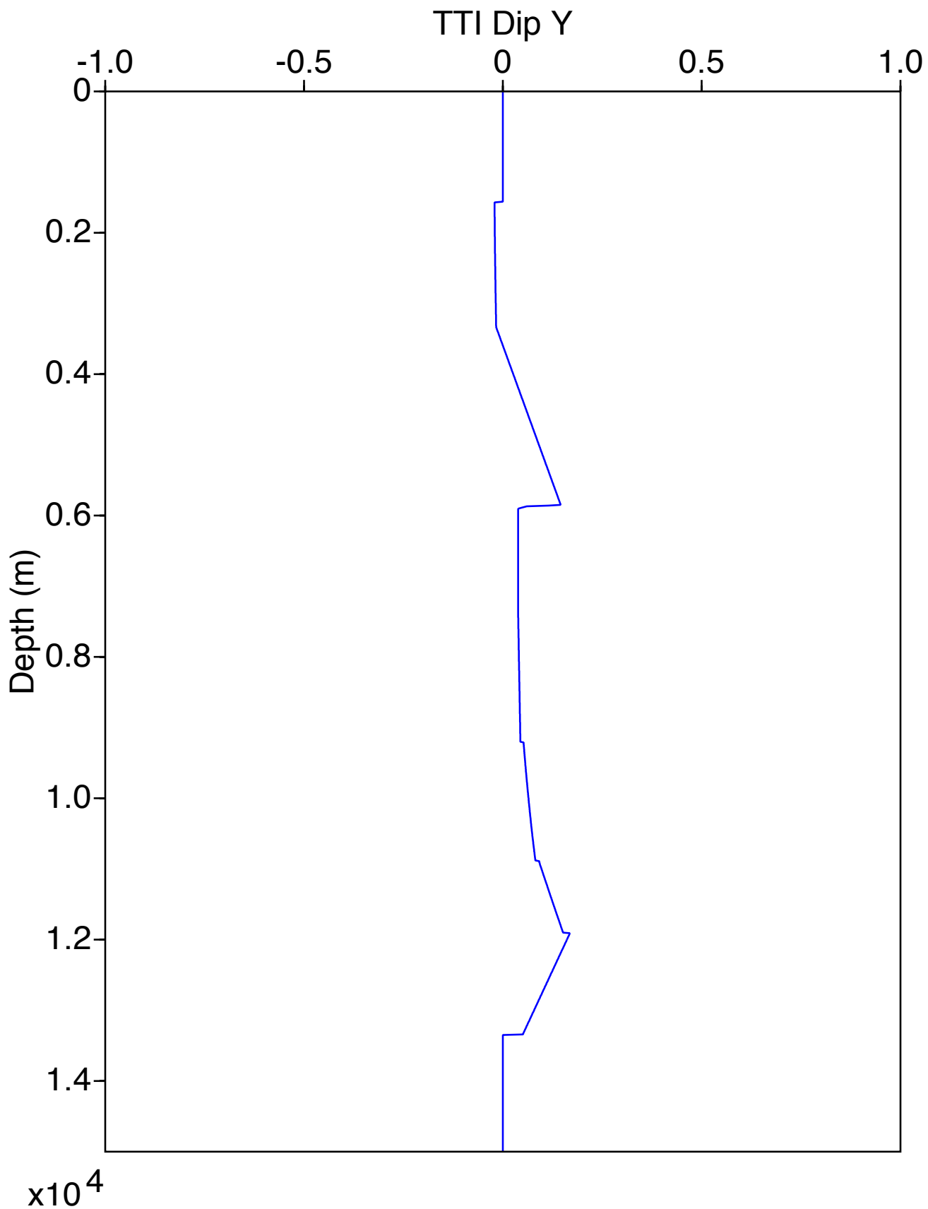
TTIDipY Log for Well 4
