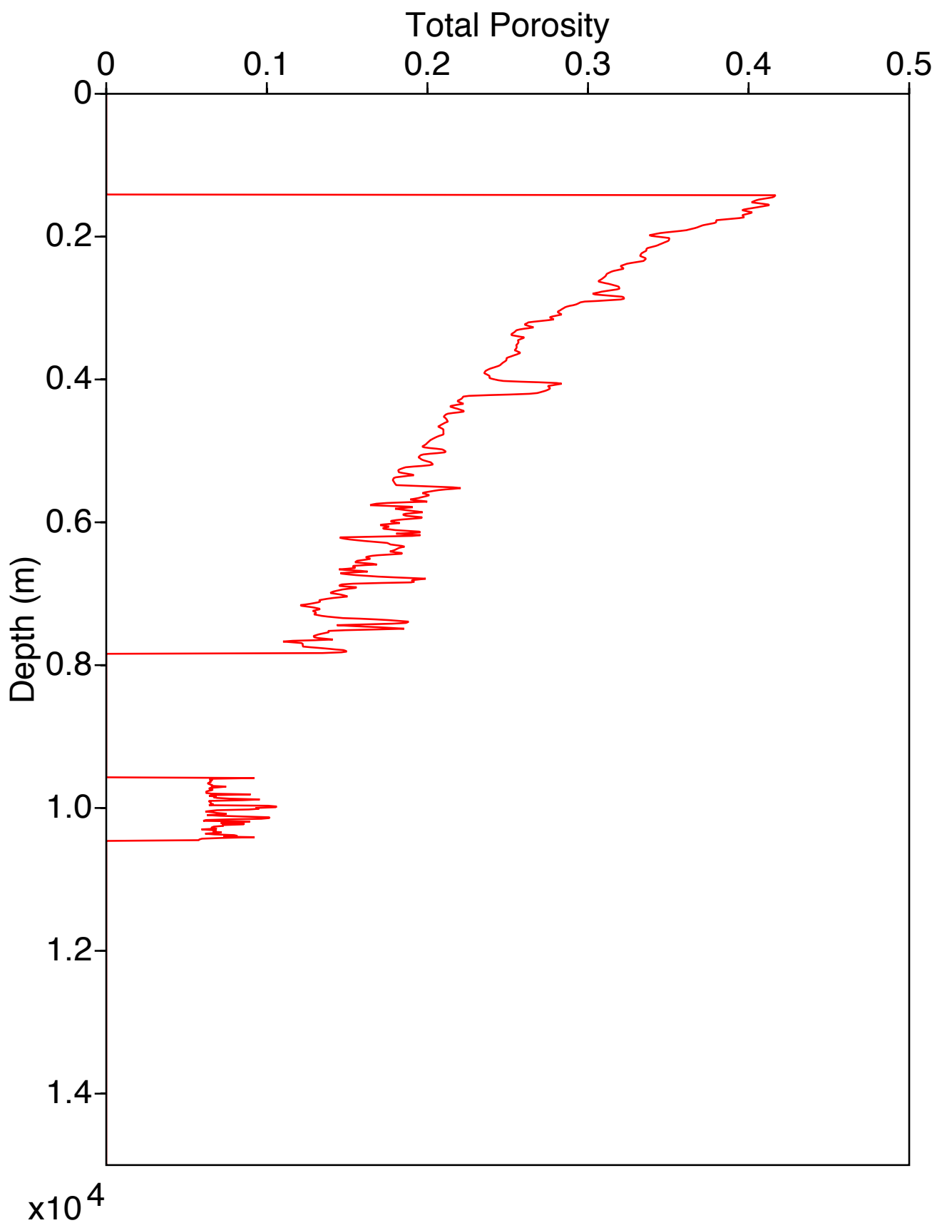
PorosityTotal Log for Well 2
