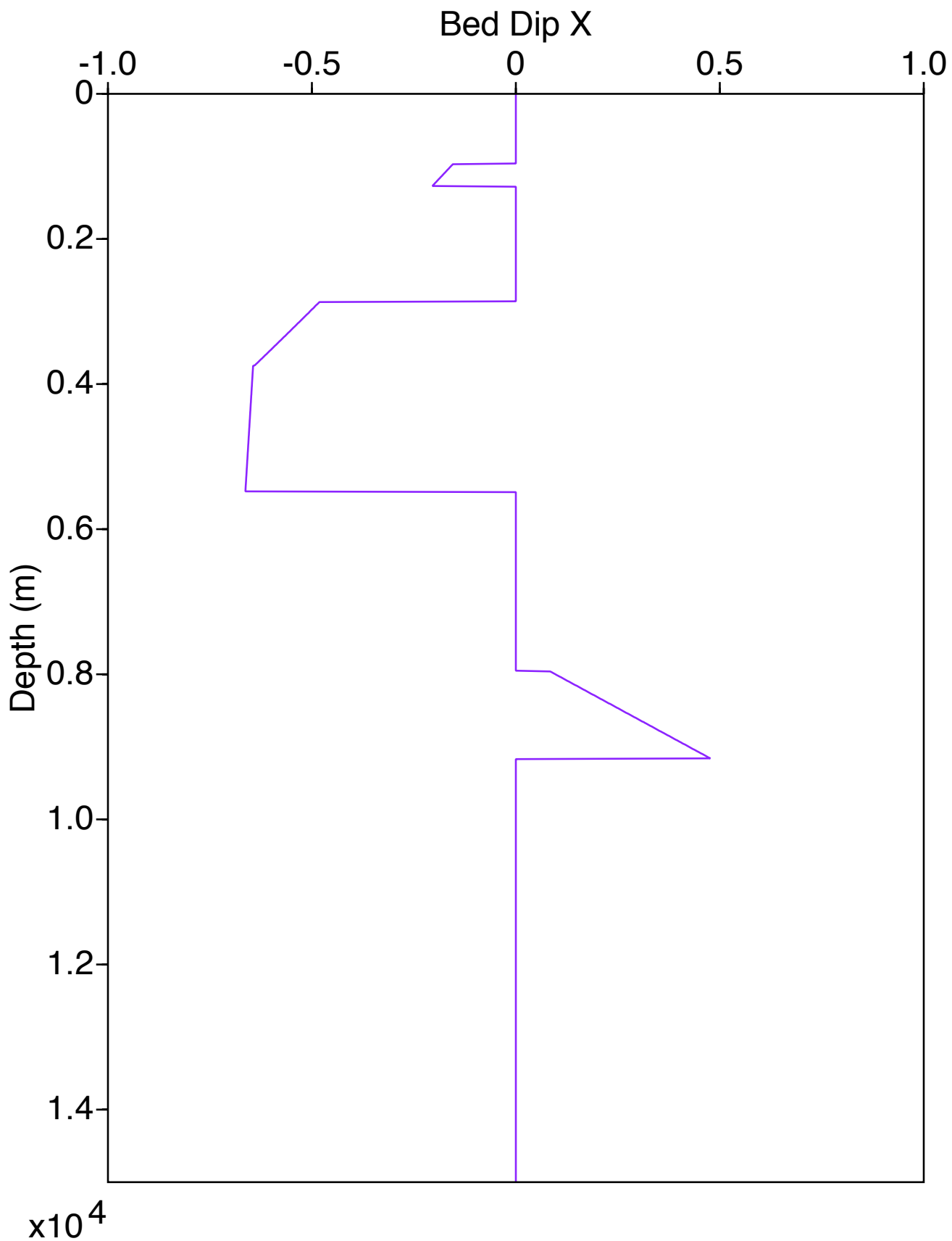
BedDipX Log for Well 5
