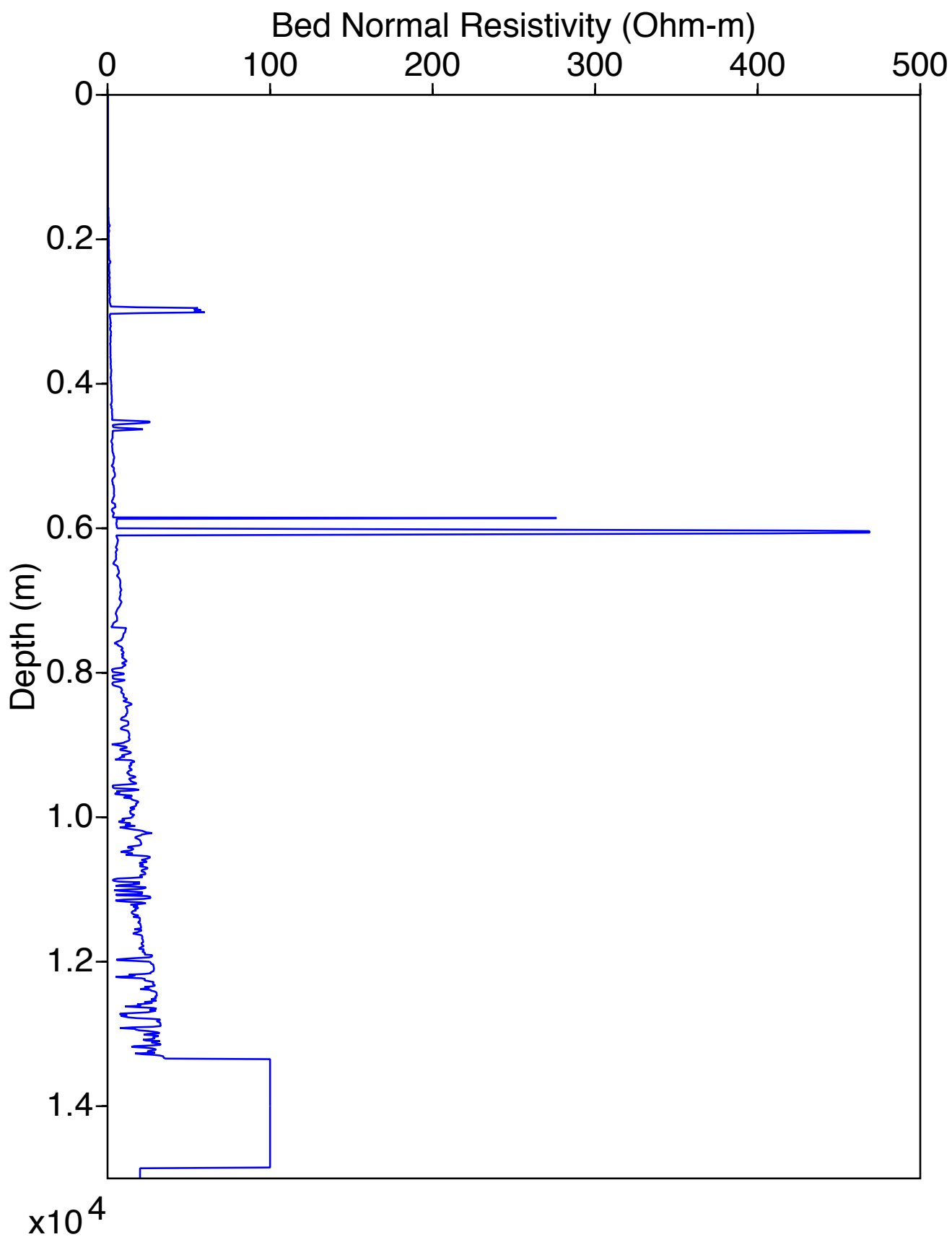
ResistivityNormal Log for Well 4
