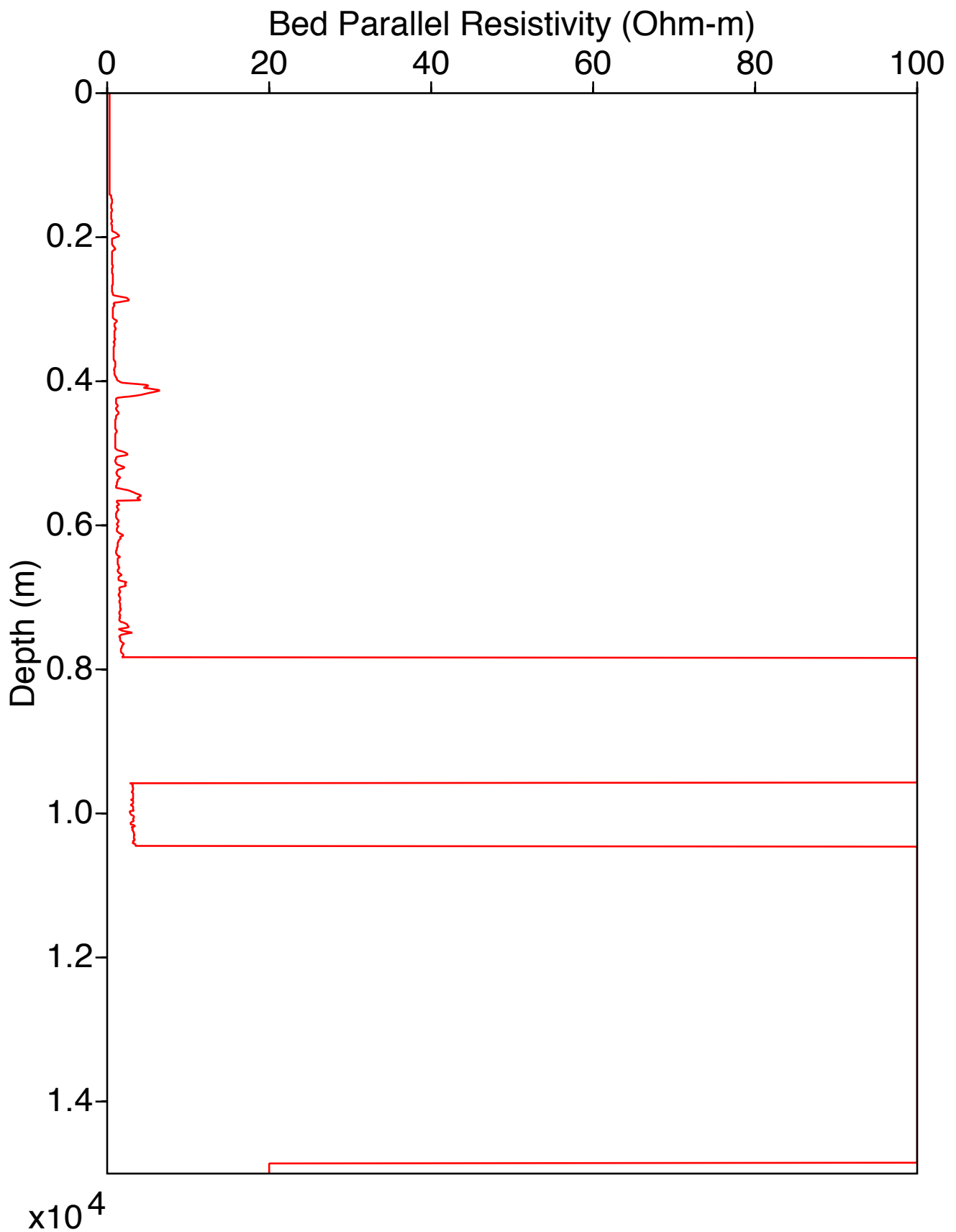
ResistivityParallel Log for Well 2
