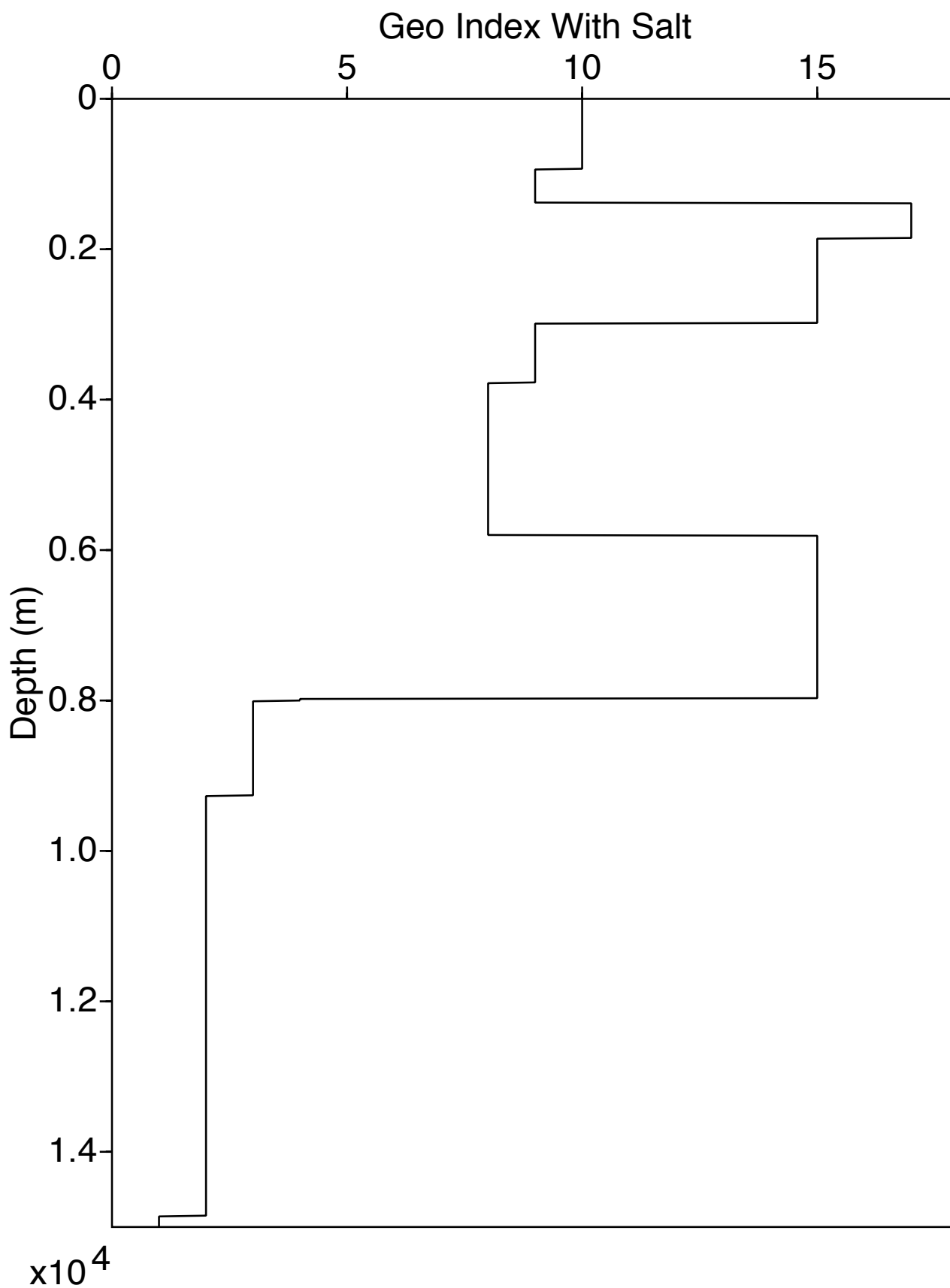
GeoSaltIndex Log for Well 3
