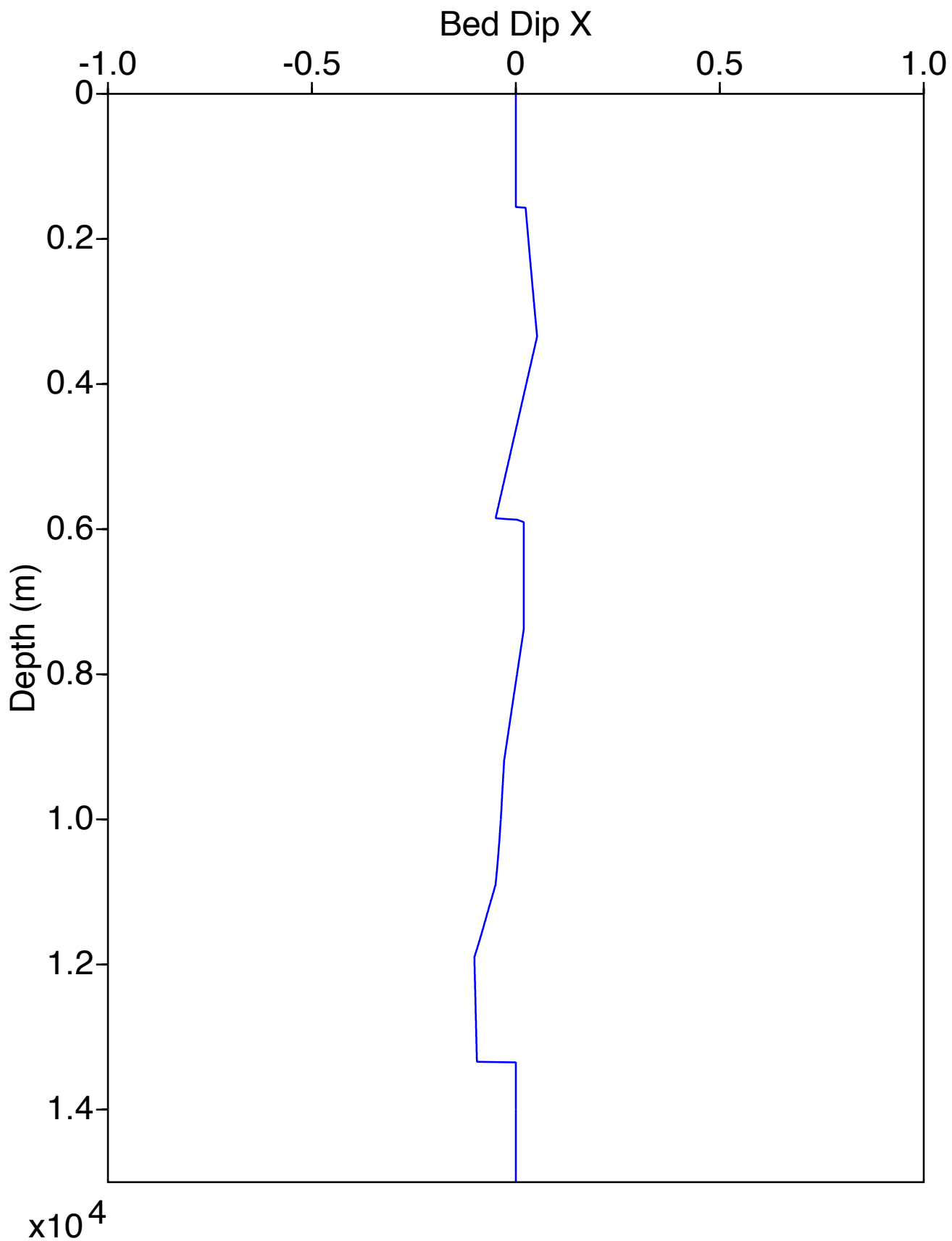
BedDipX Log for Well 4
