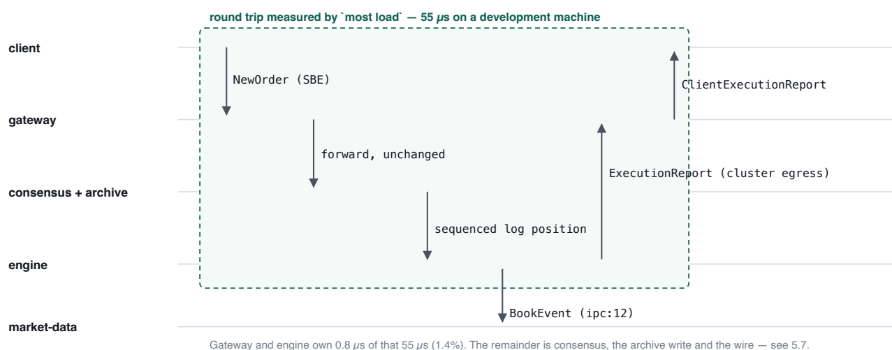
Figure 5.3 One client round trip through the stages that own it. The gateway and the engine are the two smallest.
