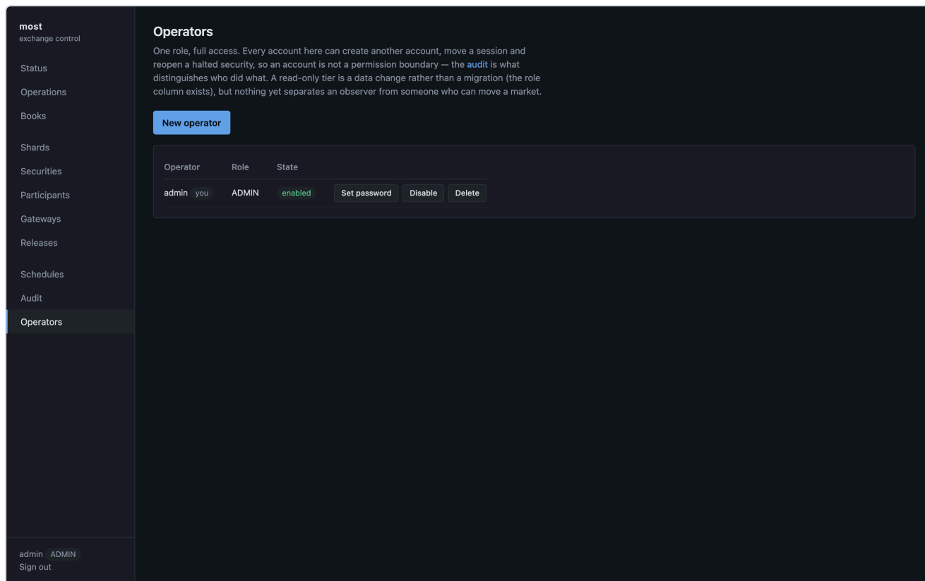
Figure 5.4 Operators. Accounts and their state. The column exists so that adding a read-only tier later is a data change rather than a migration.
