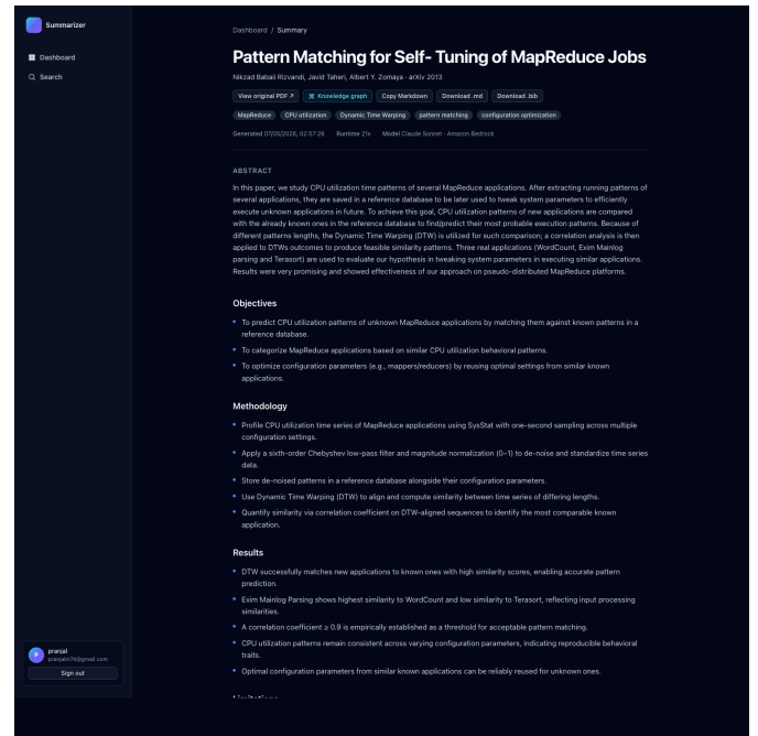
Fig. 5. Summary detail view for a real paper retrieved from arXiv. The five-section structured output (objectives, methodology, results, limitations, contributions) is produced by the SQS-triggered Step Functions pipeline and rendered directly from the get-summary endpoint.
