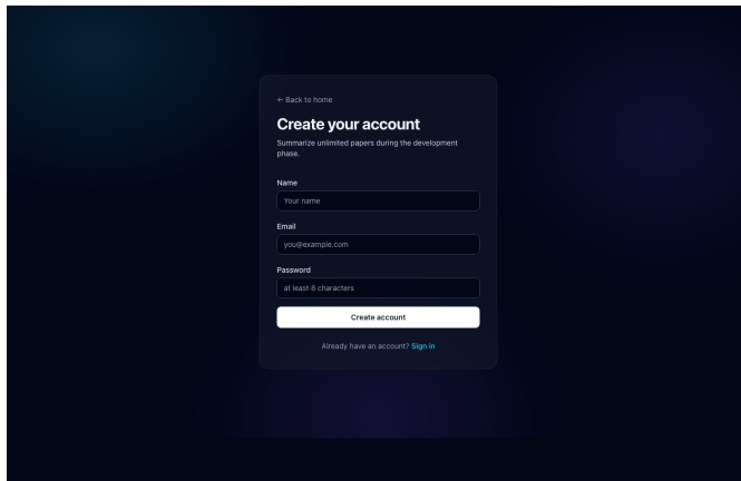
Fig. 3. Signup page wired to Amazon Cognito with email-based self-service verification.
