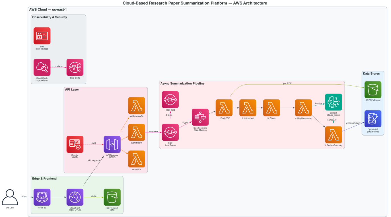
Fig. 1. System architecture. CloudFront fronts a private S3 frontend bucket and forwards dynamic traffic to API Gateway. Cognito authorizes gate every API route. The “submit job” handler enqueues to SQS; a trigger Lambda starts a Step Functions execution that orchestrates Fetch, Extract, Chunk, parallel MapSummarize, and Reduce stages. DynamoDB holds jobs and chunk embeddings; S3 holds PDFs and intermediate text. Bedrock serves both text generation and Titan v2 embeddings.
