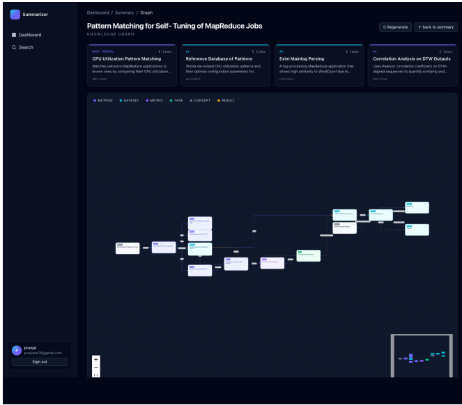
Fig. 6. Knowledge graph extracted from the structured summary. Typed entities (method, dataset, metric, task, concept, result) and relationships (uses, achieves, evaluated on, etc.) are rendered with React Flow under a left-to-right hierarchical layout, with the four most-connected entities surfaced in the key-concepts rail above the canvas.
