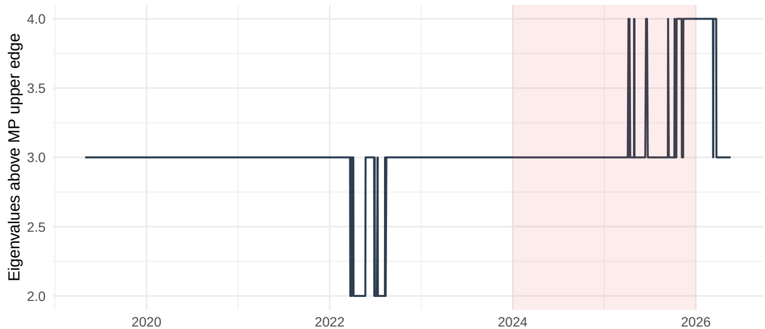
Rolling 504-day eigenvalue count (robustness: longer window)
