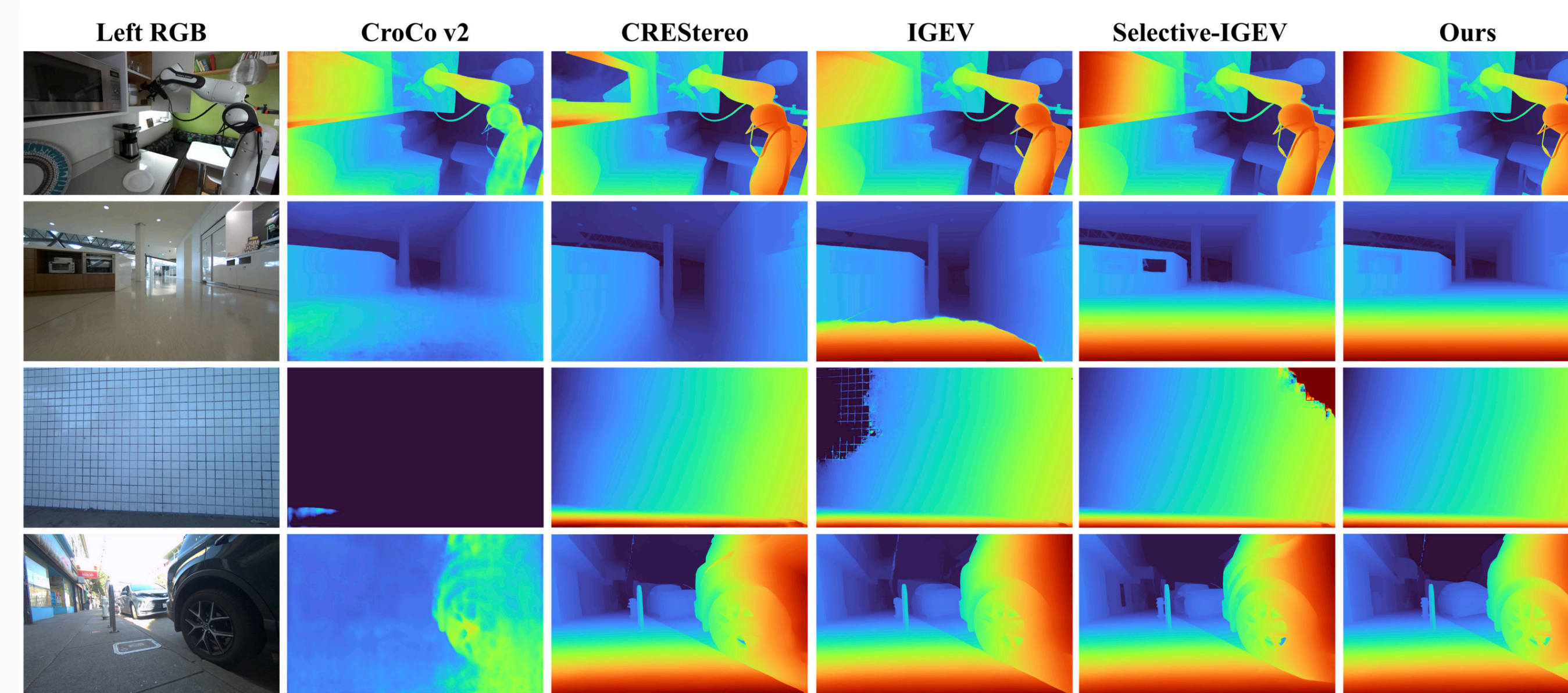
Figure 5: In-the-wild comparison
