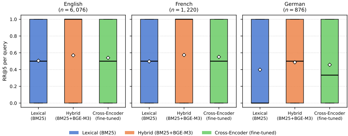
Figure 3: Per-query RR@5 distributions on the test set. Diamonds mark the per-system mean; whiskers follow the Tukey 1.5xIQR convention.
