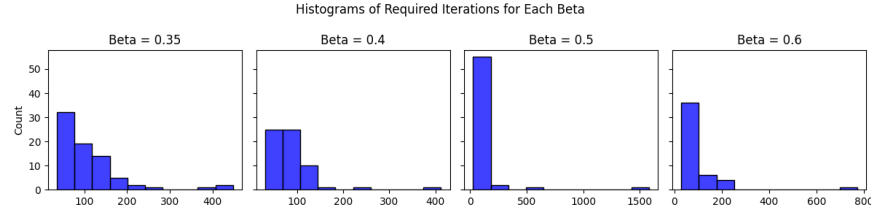
Figure 6: HNNs initialized with the empirical connectome has better convergence properties than permutation-based null models. Histograms show the number of iterations until convergence with the real (unpermuted) connectome, for 100 random initializations, with various beta values. HNN models based on the permuted connectivity matrix (with retaining symmetry) did not reach convergence in 10000 iterations in more than 98% of the same random initializations. See convergence-analysis.ipynb for details.
