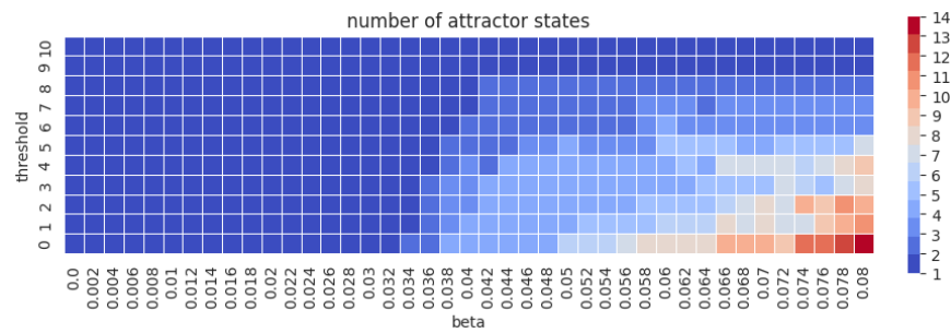
Figure 5: Parameter sweep of fcHNN parameters threshold and beta. the number of attractor states is color-coded. See supplemental_material.ipynb for details.
