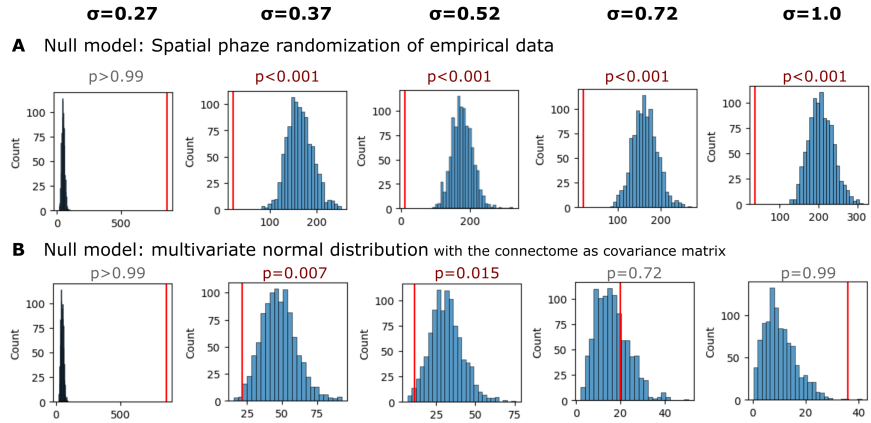
Figure 7: Statistical inference of the fcHNN state occupancy prediction with different null models. A Results with a spatial autocorrelation-preserving null model for the empirical activity patterns. See null_models.ipynb for more details. B Results where simulated samples are randomly sampled from a multivariate normal distribution, with the functional connectome as the covariance matrix, and compared to the fcHNN performance. See supplemental_material.ipynb for details.
