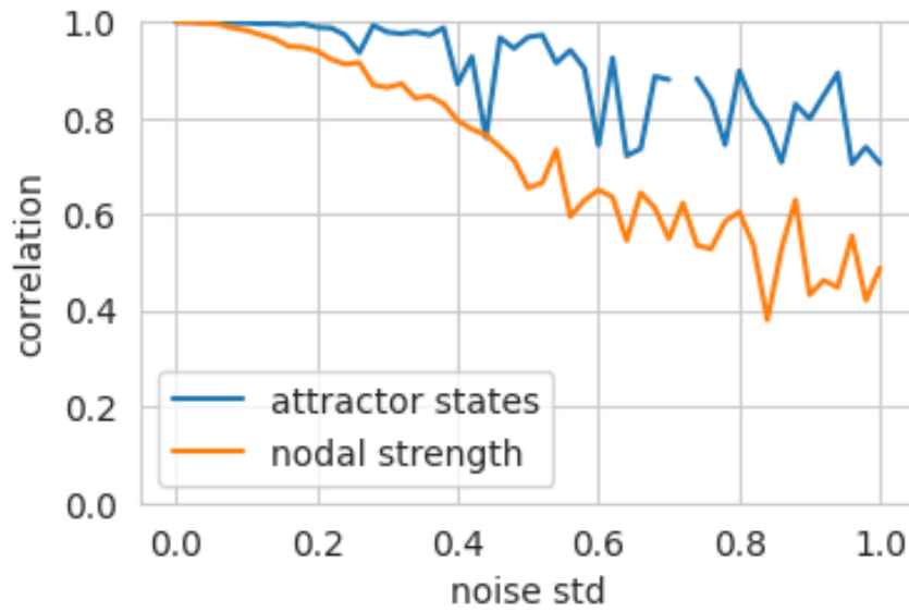
Figure 10: Robustness of the fcHNN weights to noise. We set the temperature of the fcHNN, so that two attractor states emerge and iteratively add noise to the connectome. To account for the change in dynamics, we adjust the temperature (beta) of the noisy fcHNN so that exactly two states emerge. We then highlight the decrease in nodal strength of the noisy connectome (the fcHNN weights) as a reference metric vs the correlation of the attractor states that emerge from the noisy connectome. See supplemental_material.ipynb for details.
