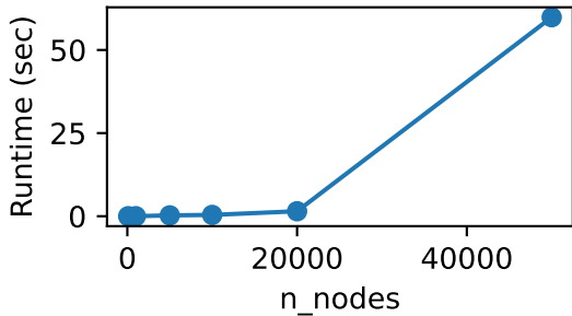
JAX Runtime vs. size
