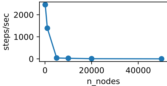
JAX throughput vs size
