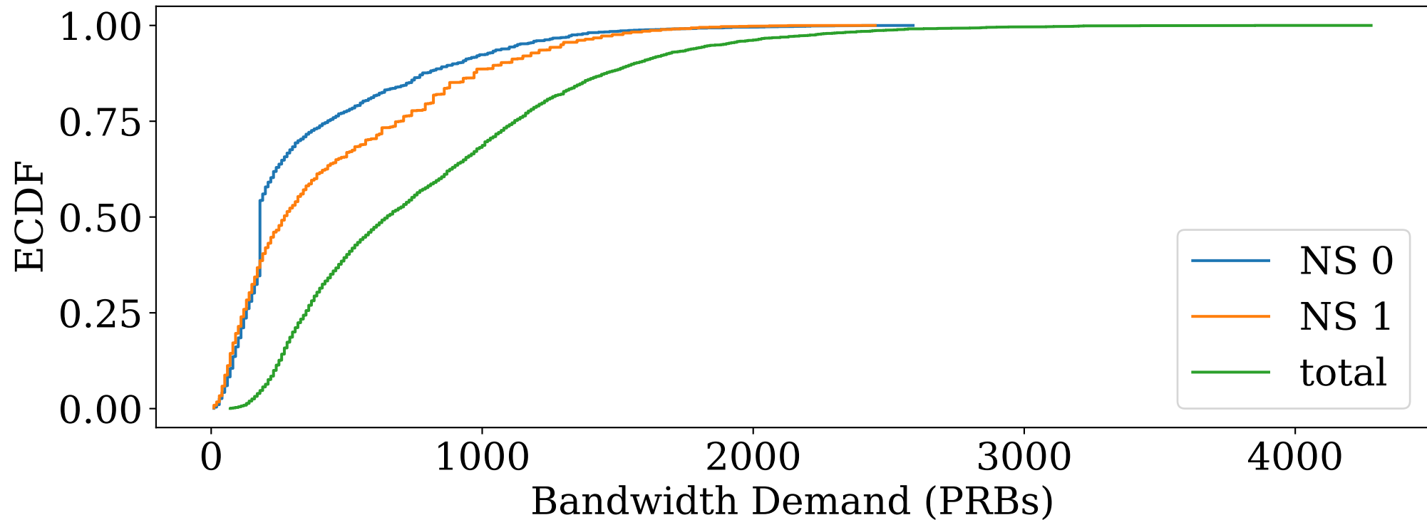
Test Scenario 2: Bandwidth Demands
