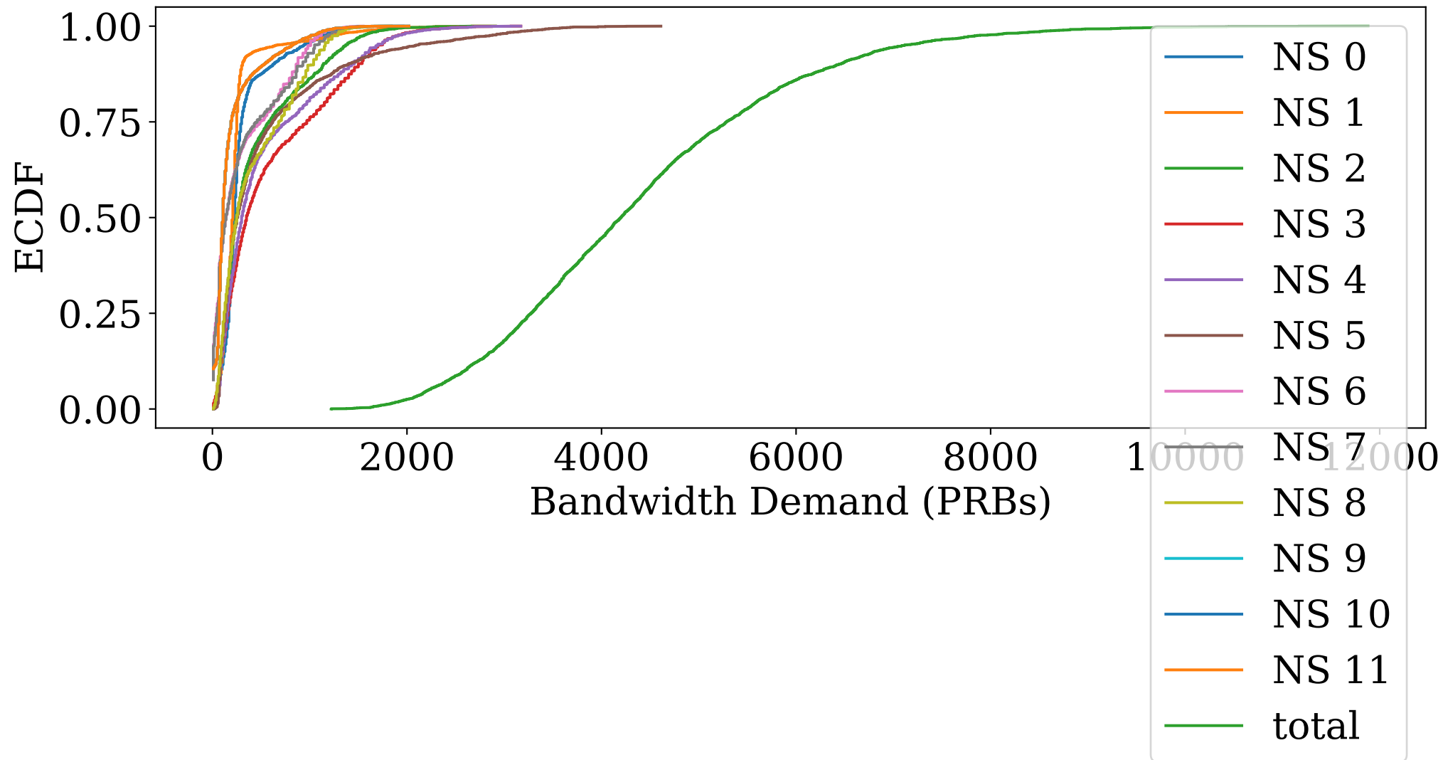
Test Scenario 4: Bandwidth Demands
