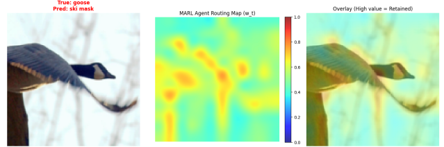
Figure 4. MARL’s saliency map
