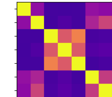
EAP
